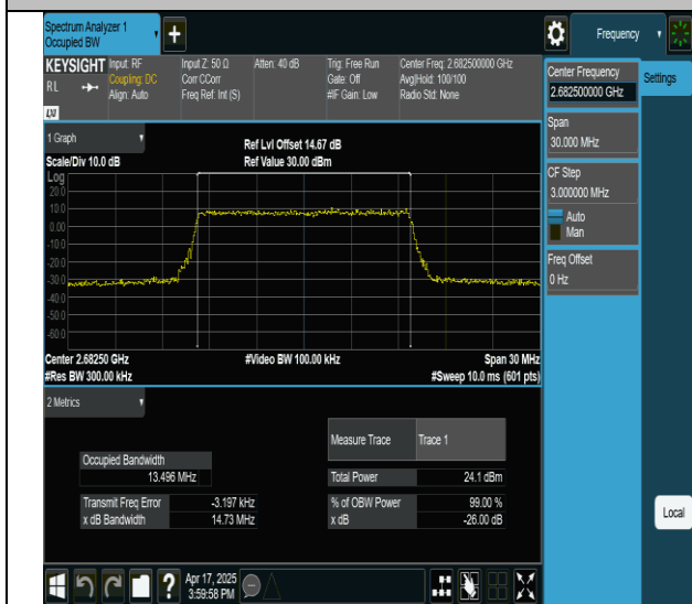
Band41-15MHz-QPSK-41515-75RB#0-PASS
