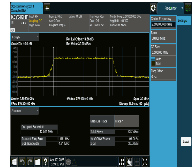
Band41-15MHz-QPSK-40620-75RB#0-PASS
