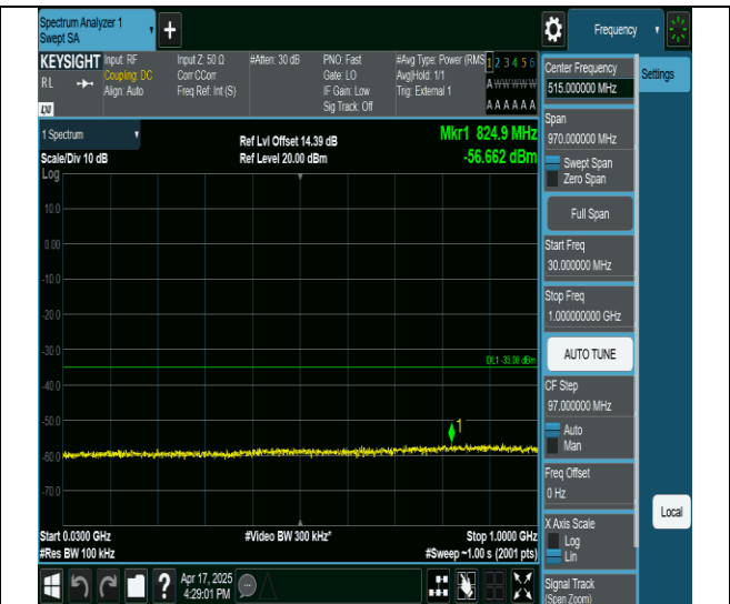
Band41-20MHz-QPSK-40620-1RB#0-30~1000-PASS
