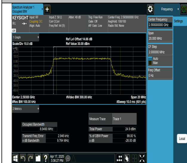
Band41-10MHz-QPSK-40620-50RB#0-PASS
