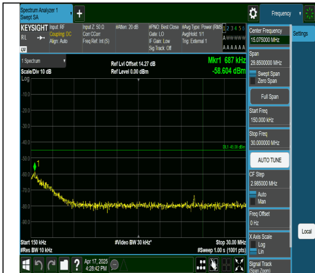
Band41-20MHz-QPSK-40620-1RB#0-0.15~30-PASS
