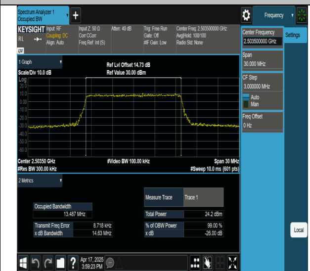
Band41-15MHz-16QAM-39725-75RB#0-PASS
