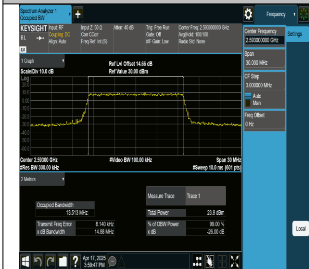
Band41-15MHz-16QAM-40620-75RB#0-PASS
