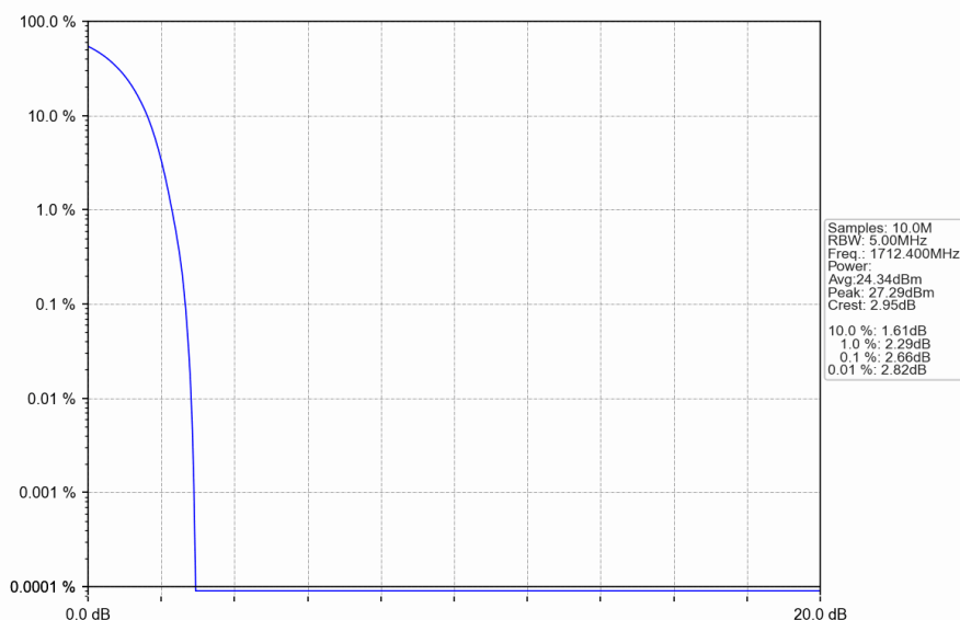
Band IV_RMC_LCH_1712.4MHz_12.2kbps RMC_NTNV
