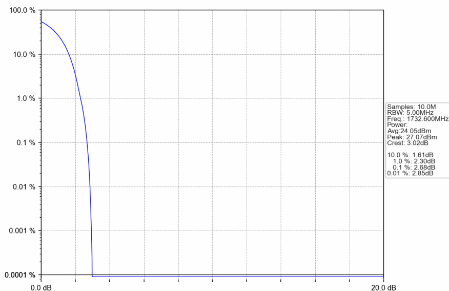
Band IV_RMC_MCH_1732.6MHz_12.2kbps RMC_NTNV
