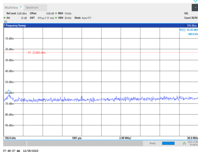
Band5-10MHz-QPSK-20450-1RB#0-Range2:0.15~30MHz
