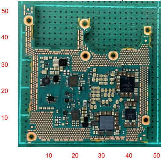
Internal Main-PWB Front (Rear-side)
