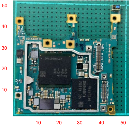
Internal Main-PWB Front without Shield cases (Front-side)
