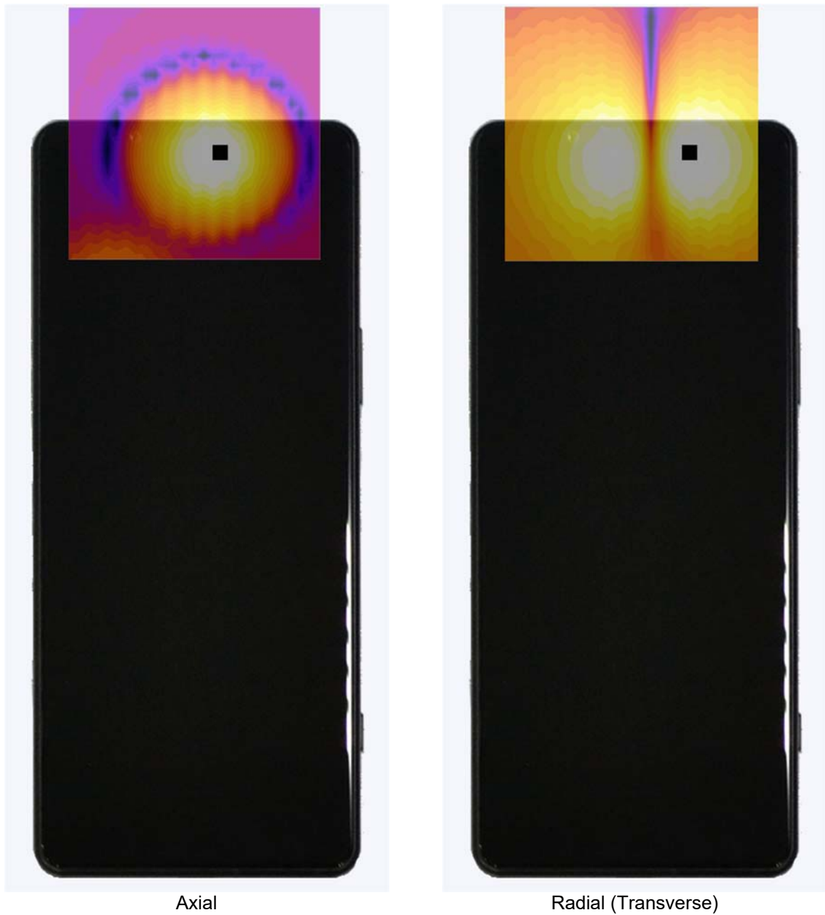
Figure 15-3 T-Coil Scan Overlay Magnetic Field Distributions
