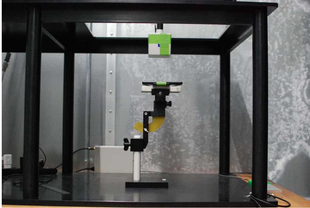
Test Setup Photo 23 H-field, Front side, 15cm
