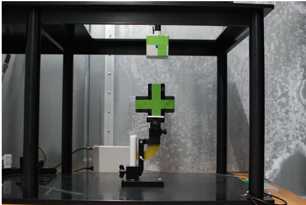
Test Setup Photo 24 H-field, Top edge, 15cm
