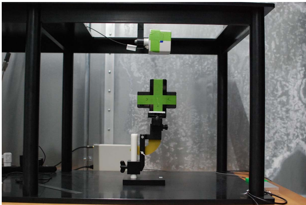
Test Setup Photo 18 E-field, Top edge, 15cm
