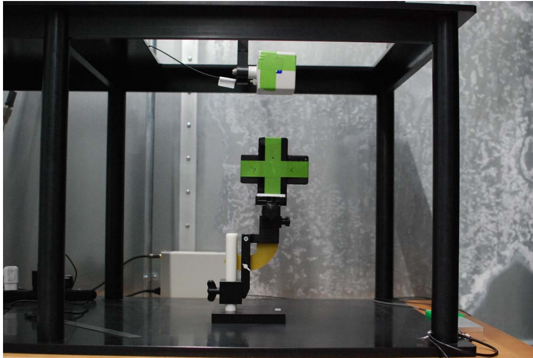
Test Setup Photo 19 E-field, Bottom edge, 15cm
