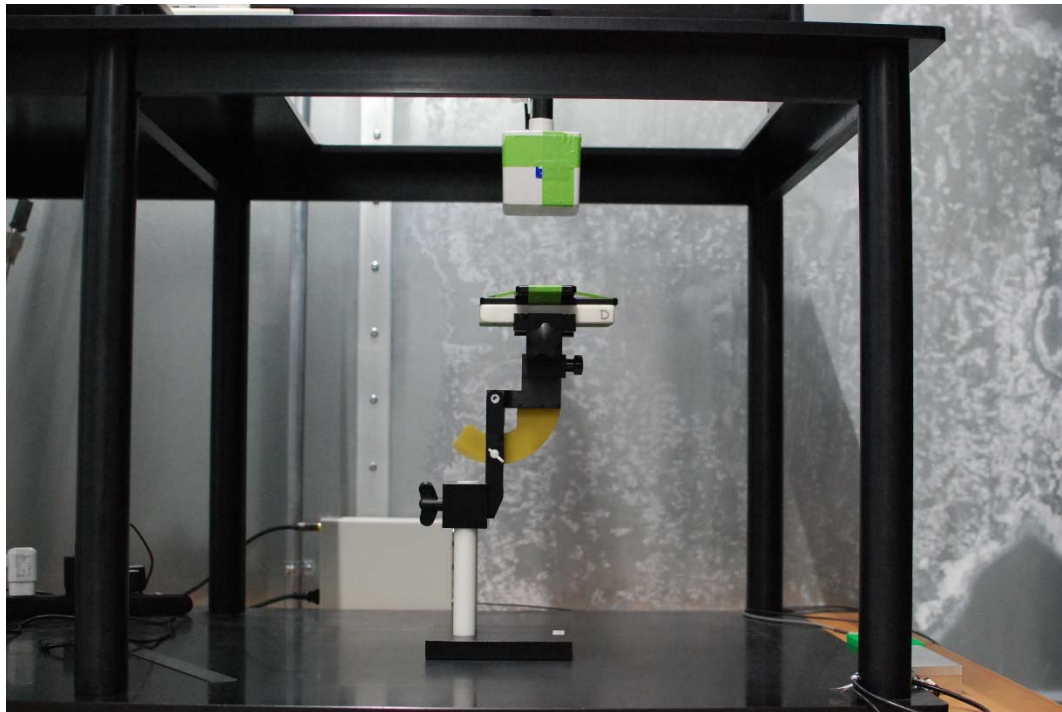
Test Setup Photo 22 H-field, Back side, 15cm
