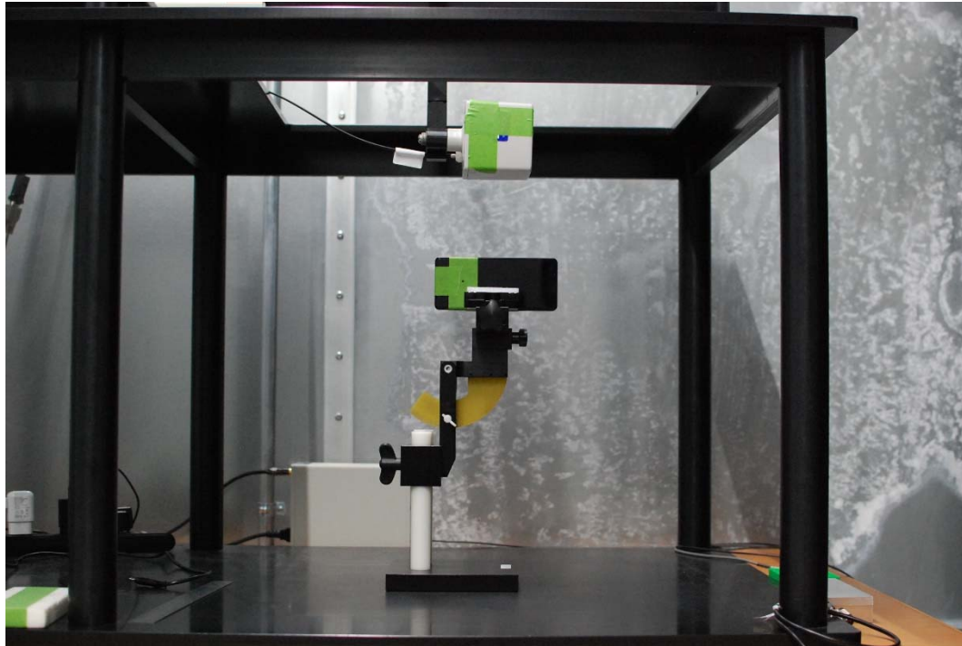
Test Setup Photo 9 E-field, Left edge, 15cm
