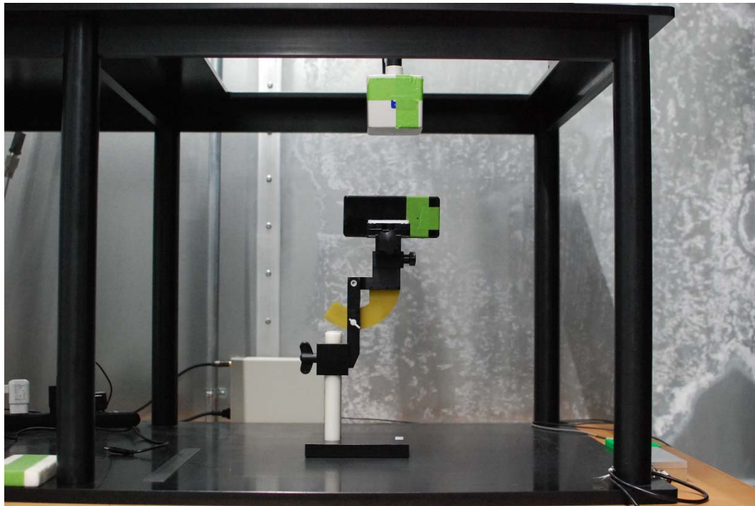
Test Setup Photo 14 H-field, Right edge, 15cm
