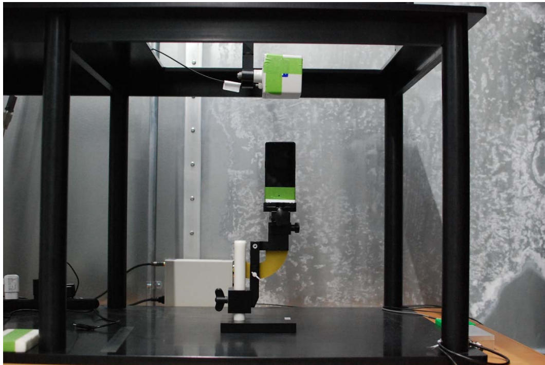
Test Setup Photo 6 E-field, Top edge, 15cm
