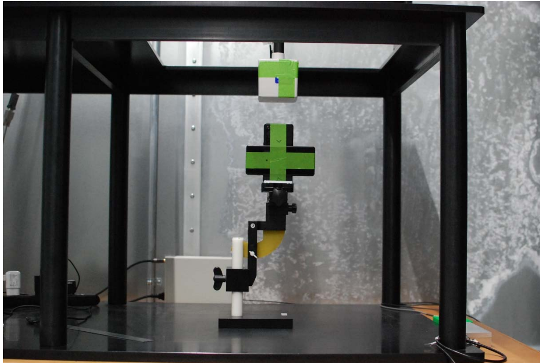
Test Setup Photo 27 H-field, Left edge, 15cm
