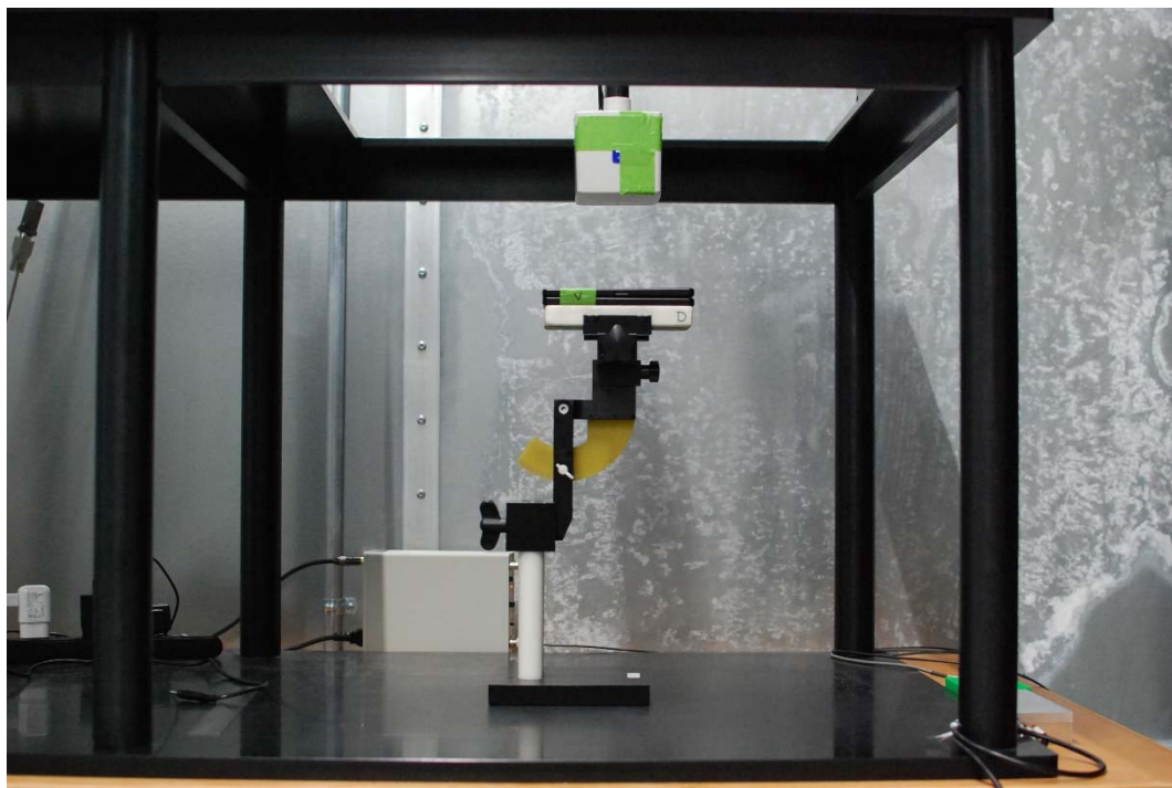
Test Setup Photo 10 H-field, Back side, 15cm
