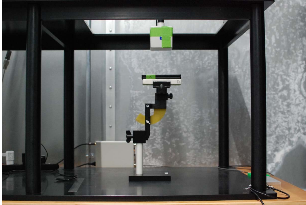
Test Setup Photo 11 H-field, Front side, 15cm
