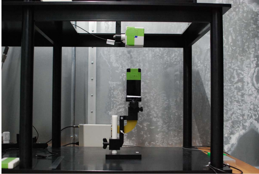
Test Setup Photo 7 E-field, Bottom edge, 15cm
