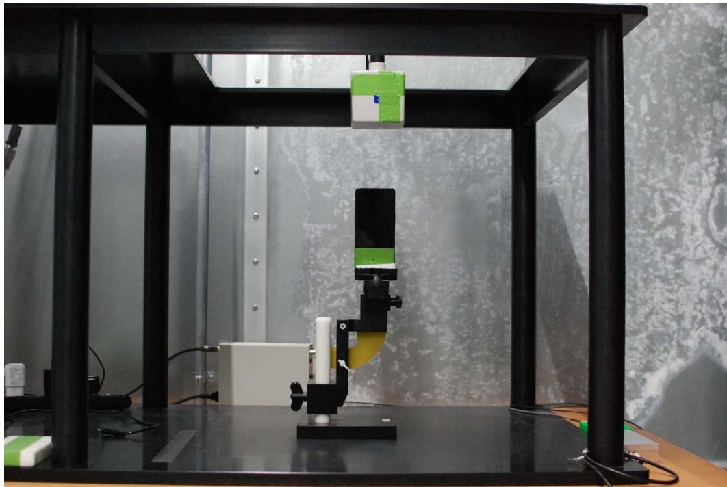
Test Setup Photo 12 H-field, Top edge, 15cm
