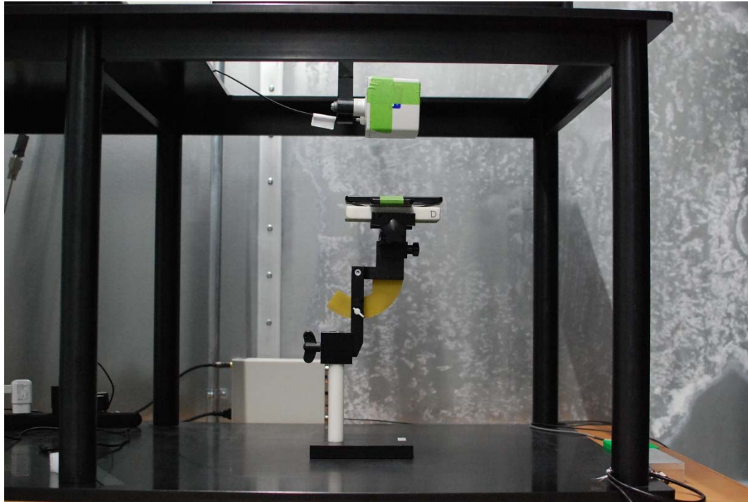
Test Setup Photo 17 E-field, Front side, 15cm
