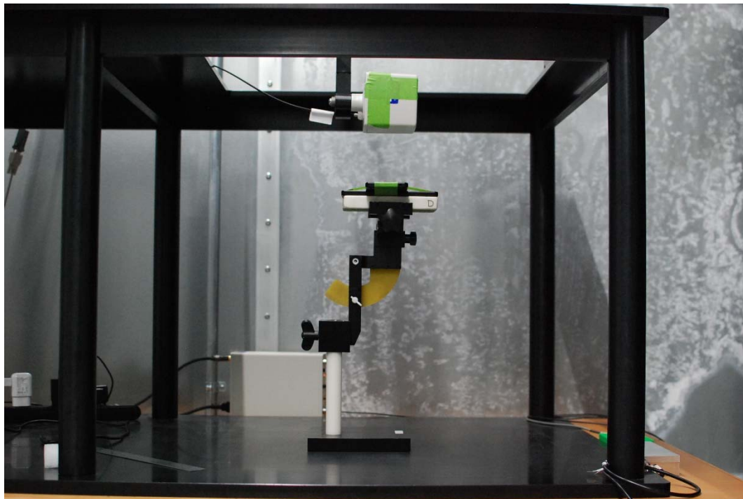
Test Setup Photo 16 E-field, Back side, 15cm
