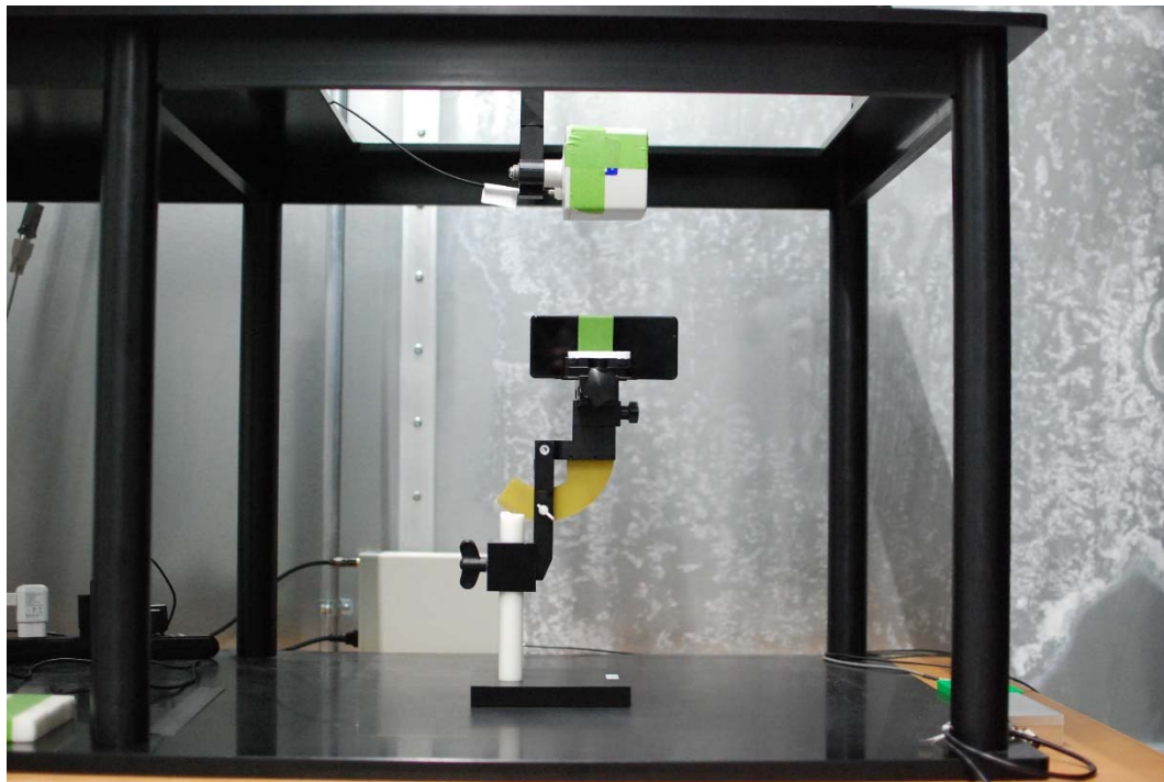
Test Setup Photo 28 E-field, Left edge, 15cm
