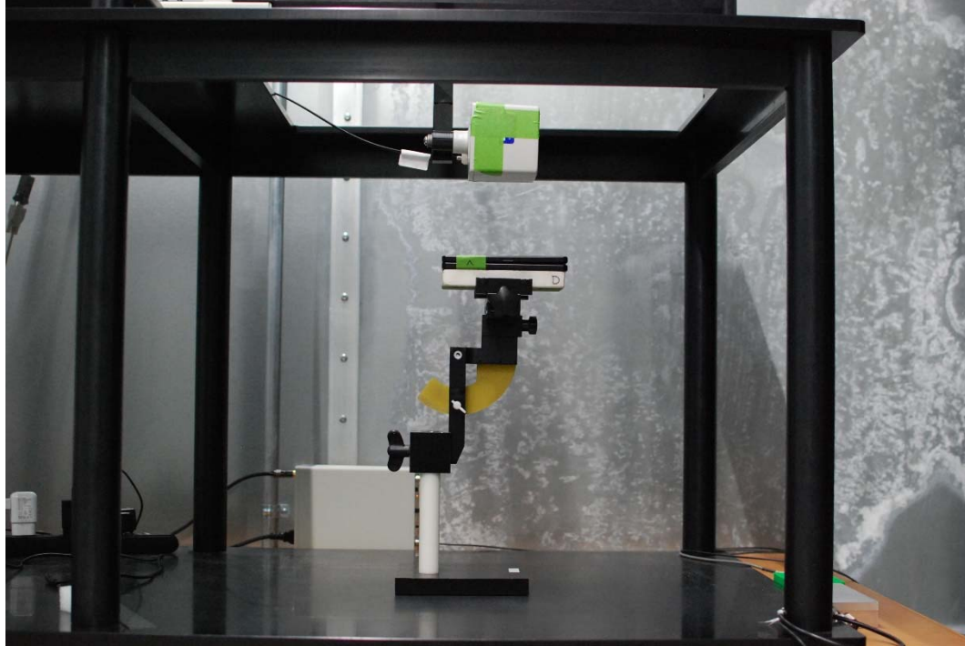
Test Setup Photo 5 E-field, Front side, 15cm
