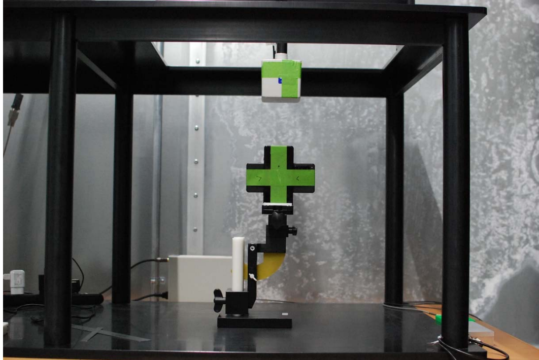
Test Setup Photo 25 H-field, Bottom edge, 15cm
