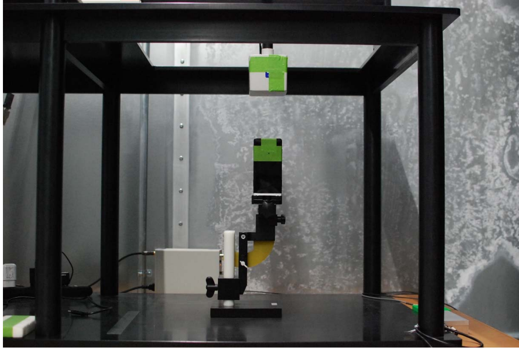
Test Setup Photo 13 H-field, Bottom edge, 15cm
