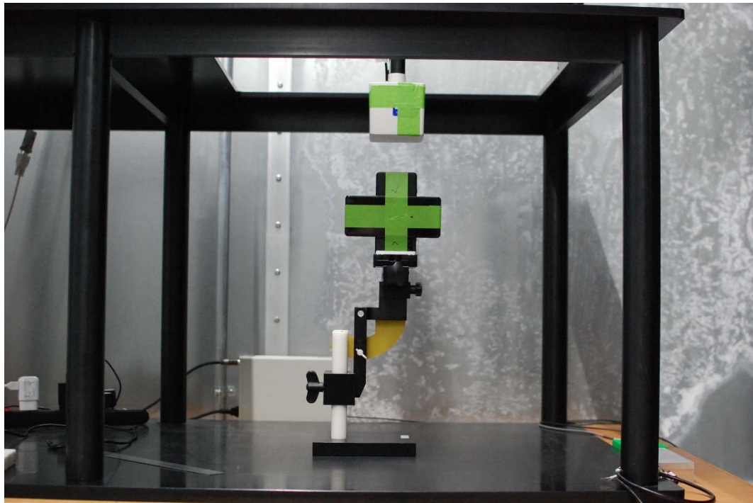
Test Setup Photo 26 H-field, Right edge, 15cm
