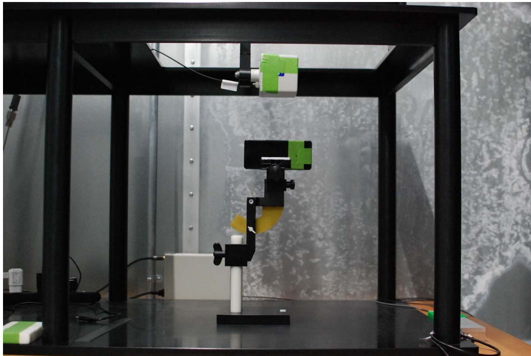
Test Setup Photo 8 E-field, Right edge, 15cm
