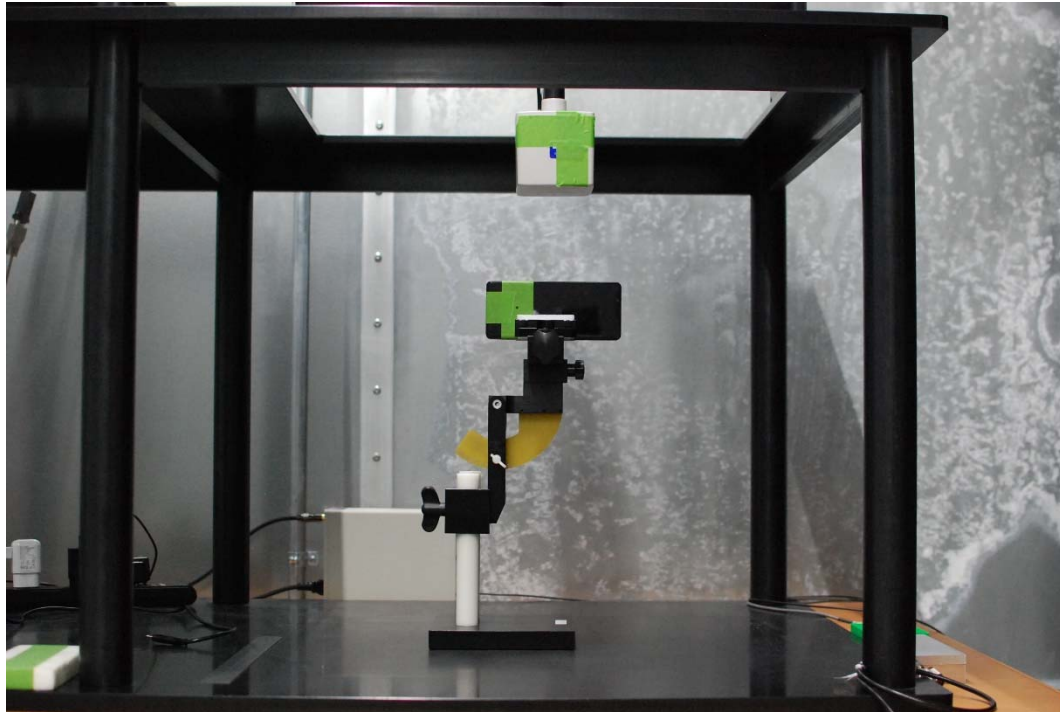
Test Setup Photo 15 H-field, Left edge, 15cm
