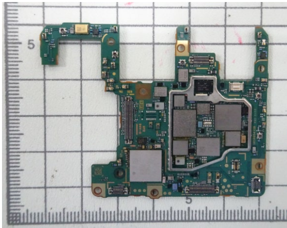
Rear PBA without Shield case (Front-side)
