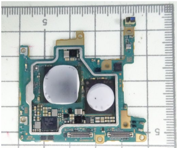
Front PBA without Shield cases (Front-side)
