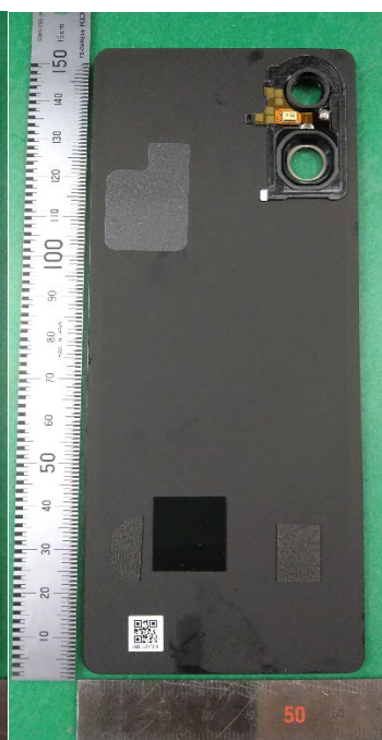
Rear panel
