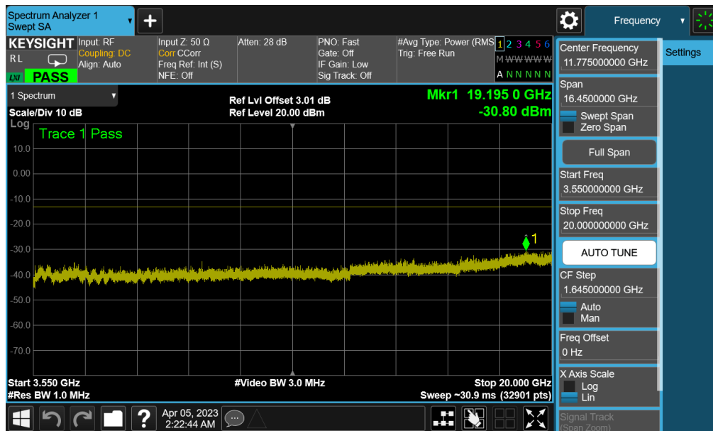
Plot 7-101. Conducted Spurious Plot (NR Band n77 PC3 (DoD) - 100MHz QPSK - 1RB - Mid Channel - Sub-UHB (UL-MIMO))
