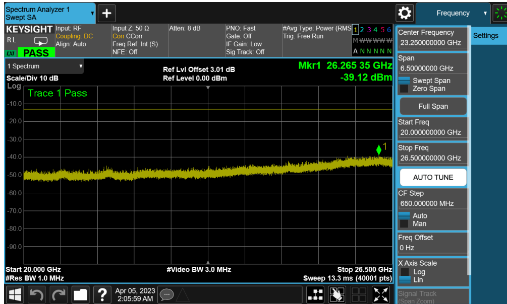
Plot 7-111. Conducted Spurious Plot (NR Band n77 PC3 (C-band) - 100MHz QPSK - 1RB - Low Channel - Main1 (UL-MIMO))
