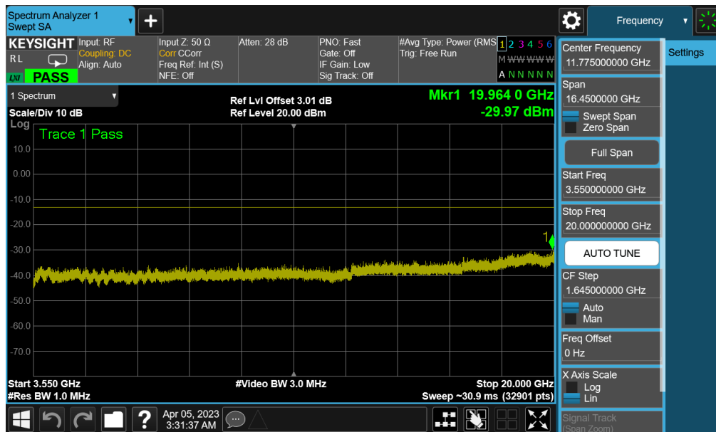
Plot 7-107. Conducted Spurious Plot (NR Band n77 PC3 (DoD) - 100MHz QPSK - 1RB - Mid Channel - 4th-MHB (SRS 2T4R))
