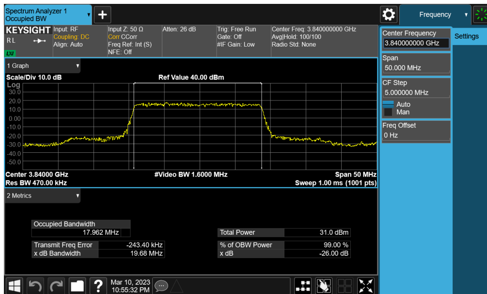
Plot 7-92. Occupied Bandwidth Plot (NR Band n77 PC2 (C-band) - 20MHz \pi/2 BPSK - Full RB - Sub-UHB)
