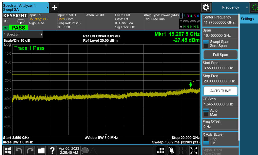
Plot 7-98. Conducted Spurious Plot (NR Band n77 PC3 (DoD) - 100MHz QPSK - 1RB - Mid Channel - Main1 (UL-MIMO))
