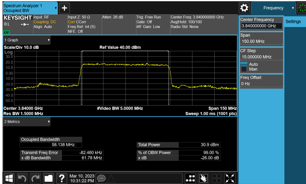
Plot 7-77. Occupied Bandwidth Plot (NR Band n77 PC2 (C-band) - 60MHz \pi/2 BPSK - Full RB - Sub-UHB)
