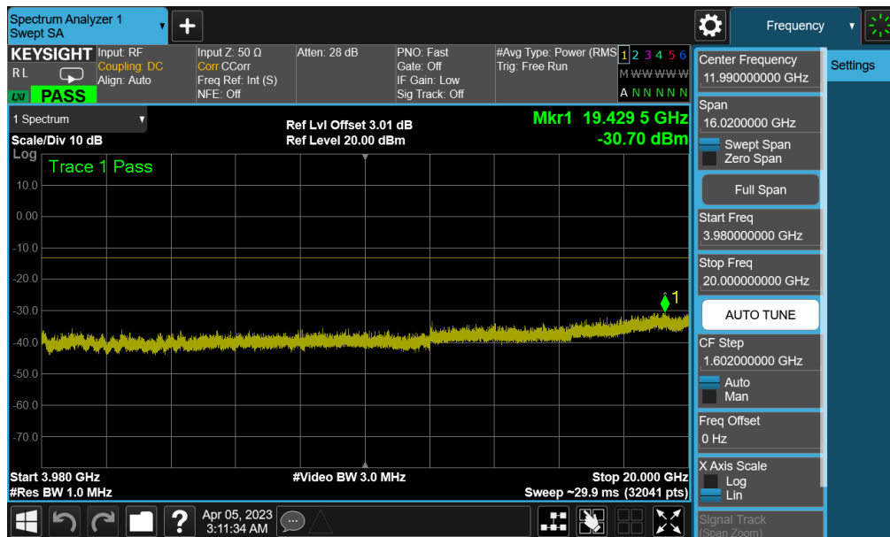
Plot 7-128. Conducted Spurious Plot (NR Band n77 PC3 (C-band) - 100MHz QPSK - 1RB - Low Channel - 3rd-LMHB (SRS 2T4R))
