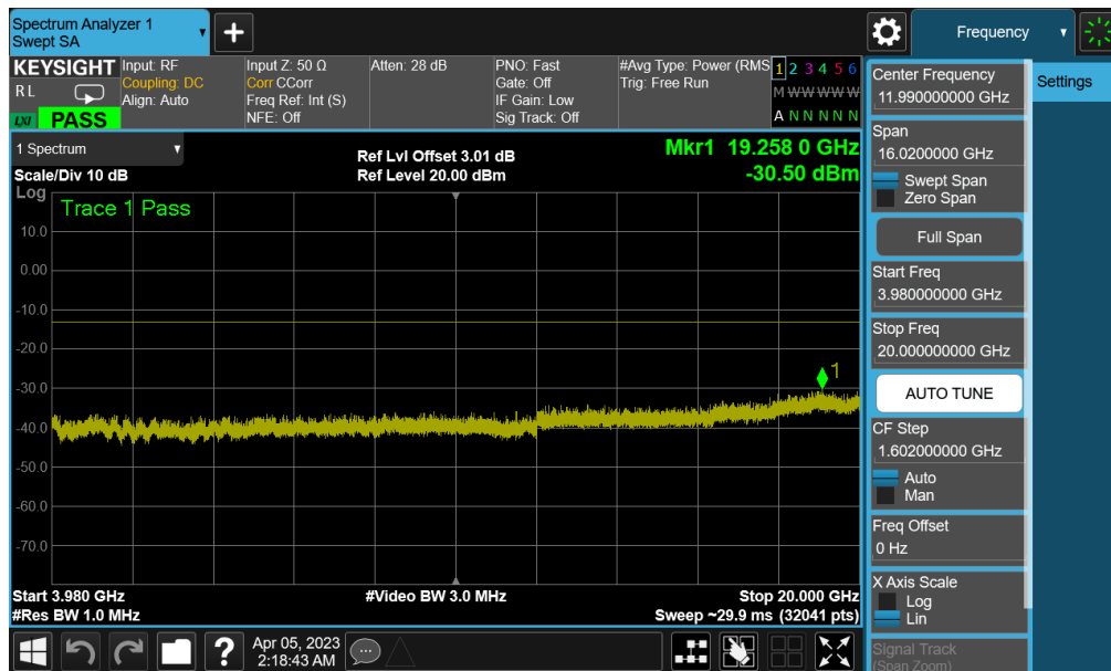
Plot 7-119. Conducted Spurious Plot (NR Band n77 PC3 (C-band) - 100MHz QPSK - 1RB - Low Channel - Sub-UHB (UL-MIMO))
