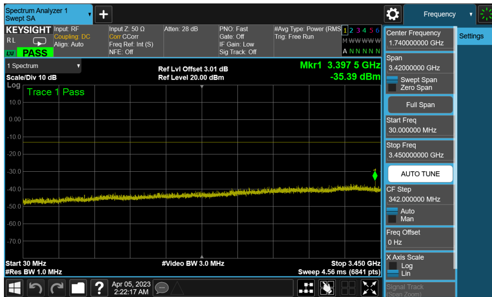
Plot 7-100. Conducted Spurious Plot (NR Band n77 PC3 (DoD) - 100MHz QPSK - 1RB - Mid Channel - Sub-UHB (UL-MIMO))
