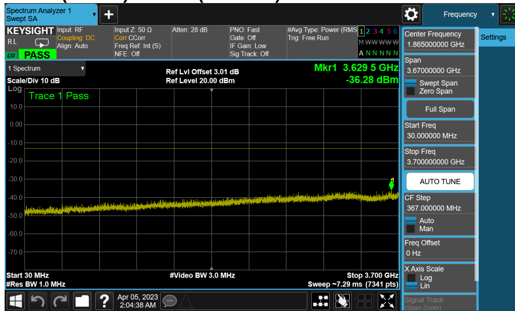
Plot 7-109. Conducted Spurious Plot (NR Band n77 PC3 (C-band) - 100MHz QPSK - 1RB - Low Channel - Main1 (UL-MIMO))
