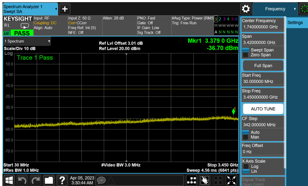
Plot 7-106. Conducted Spurious Plot (NR Band n77 PC3 (DoD) - 100MHz QPSK - 1RB - Mid Channel - 4th-MHB (SRS 2T4R))
