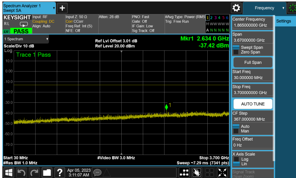
Plot 7-127. Conducted Spurious Plot (NR Band n77 PC3 (C-band) - 100MHz QPSK - 1RB - Low Channel - 3rd-LMHB (SRS 2T4R))
