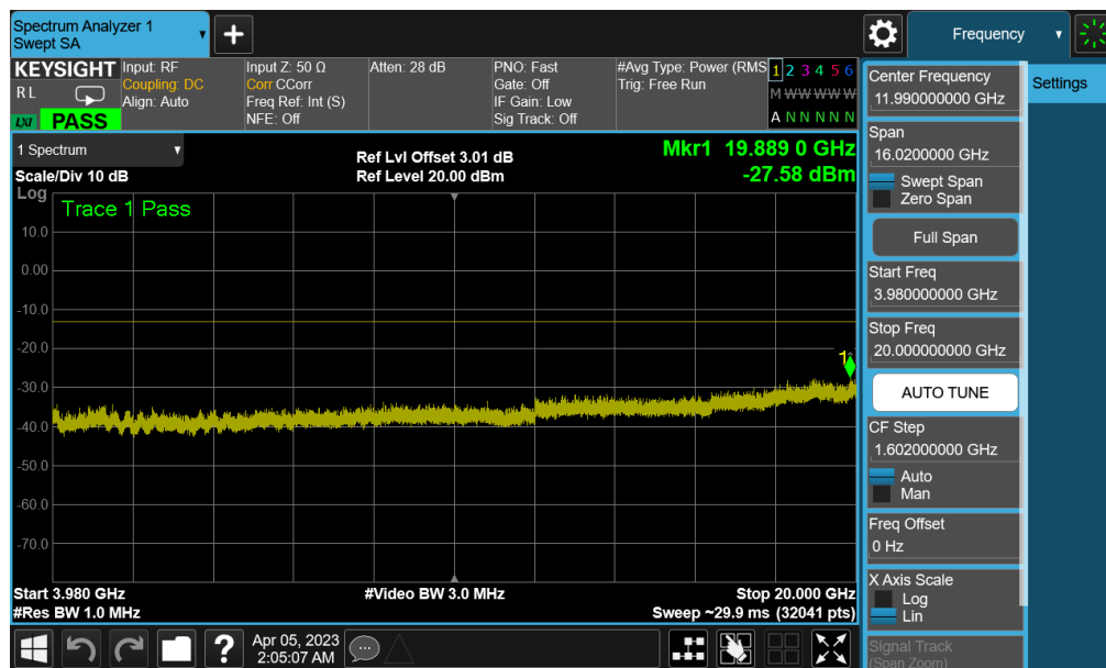
Plot 7-110. Conducted Spurious Plot (NR Band n77 PC3 (C-band) - 100MHz QPSK - 1RB - Low Channel - Main1 (UL-MIMO))
