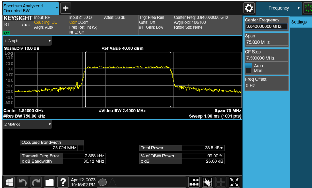
Plot 7-91. Occupied Bandwidth Plot (NR Band n77 PC2 (C-band) - 30MHz 256-QAM - Full RB - Sub-UHB)
