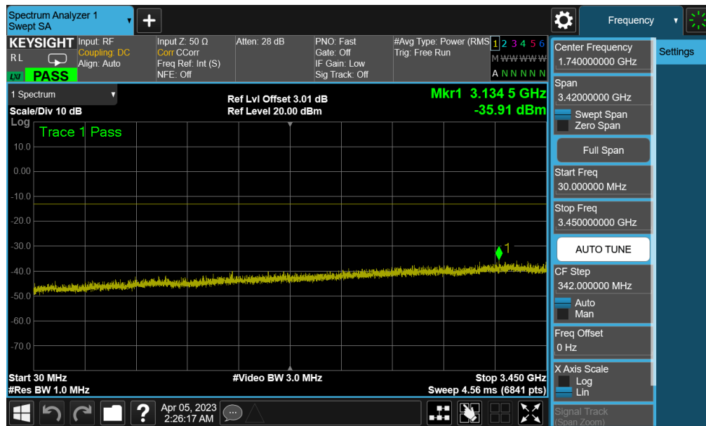
Plot 7-97. Conducted Spurious Plot (NR Band n77 PC3 (DoD) - 100MHz QPSK - 1RB - Mid Channel - Main1 (UL-MIMO))
