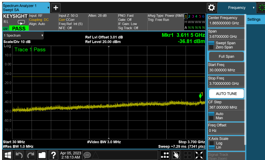
Plot 7-118. Conducted Spurious Plot (NR Band n77 PC3 (C-band) - 100MHz QPSK - 1RB - Low Channel - Sub-UHB (UL-MIMO))
