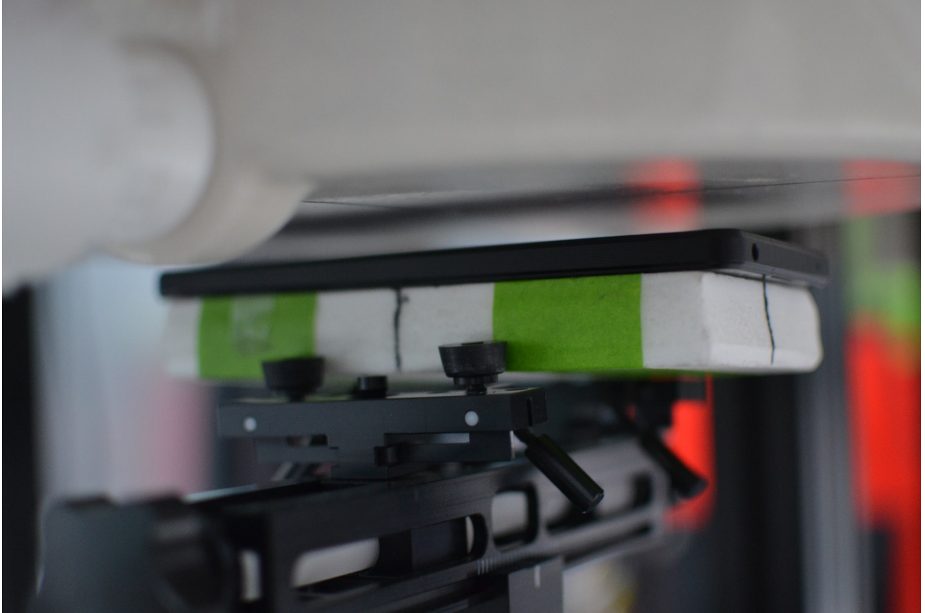
Figure F-7 SAR Test Setup Photo – Bodyworn, Back Side at 10 mm
