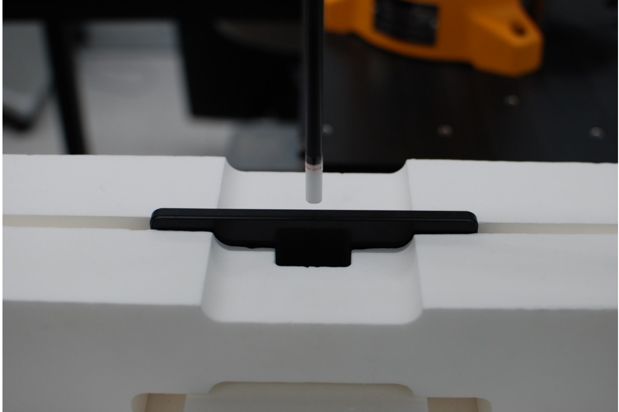
Figure F-19 Near Field Power Density Test Setup Photo – Left Edge at 9.51 mm
