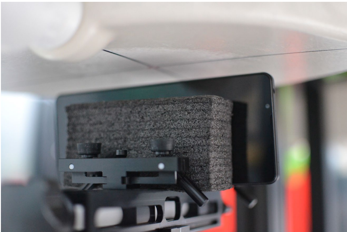
SAR Test Setup Photo 14 – Hotspot, Left Edge at 10mm
