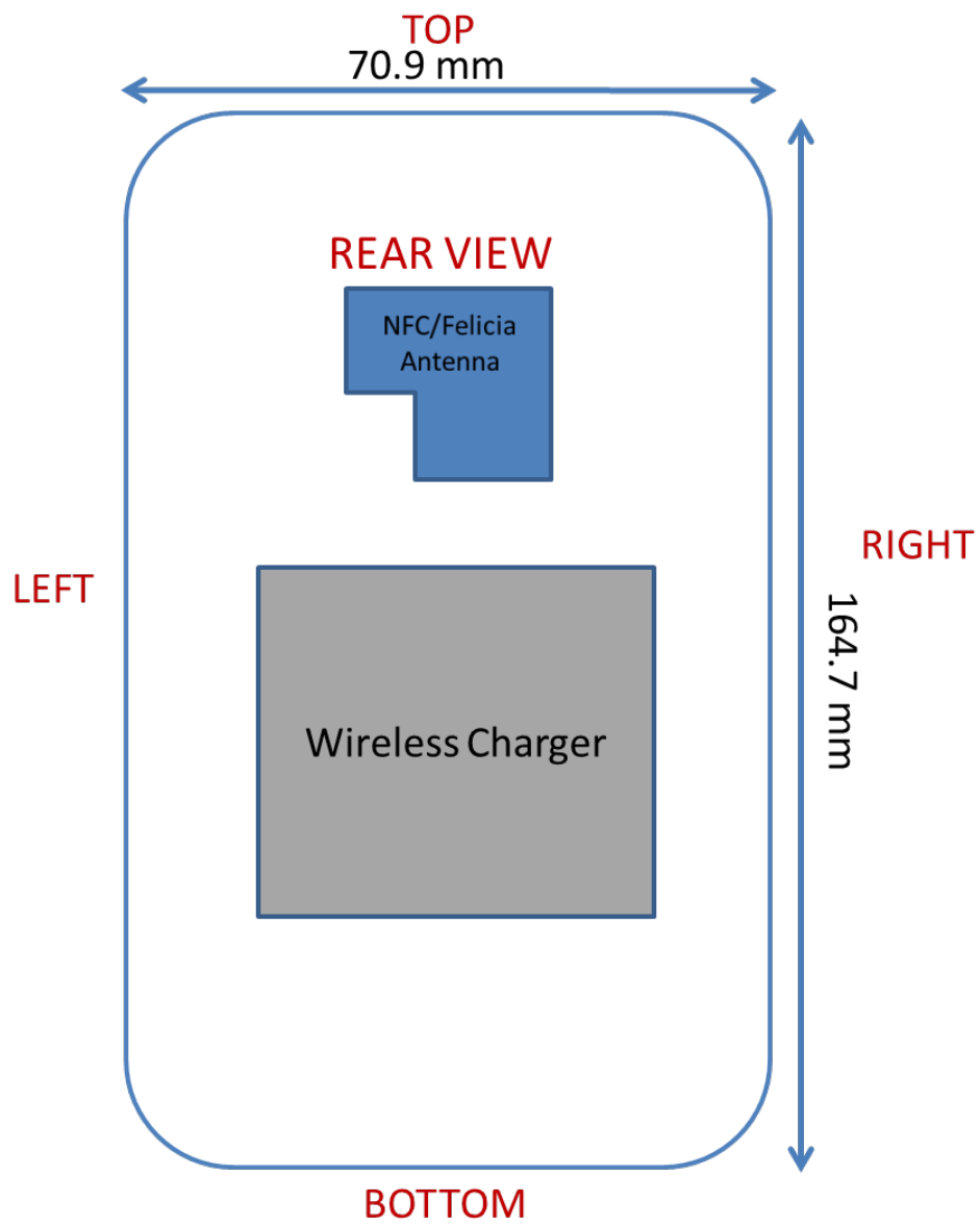
Figure J-2 NFC Antenna Locations
