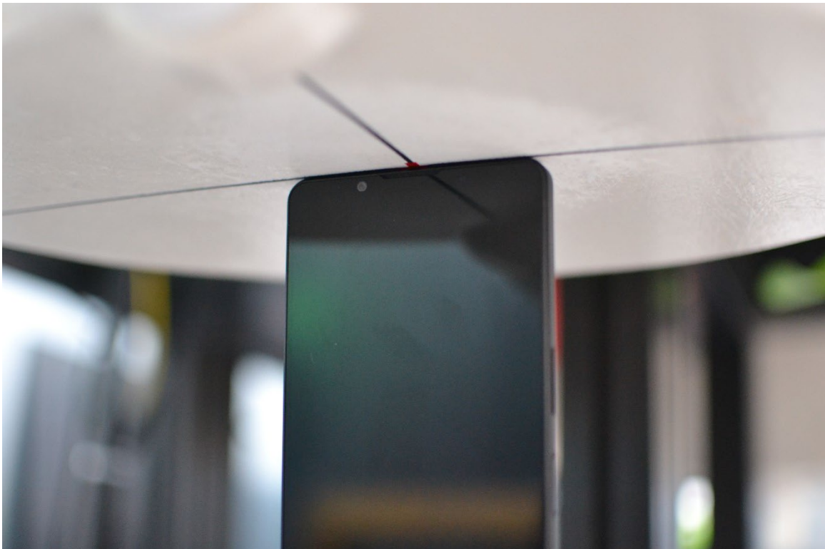
SAR Test Setup Photo 10 – Phablet, Top Edge at 0mm
