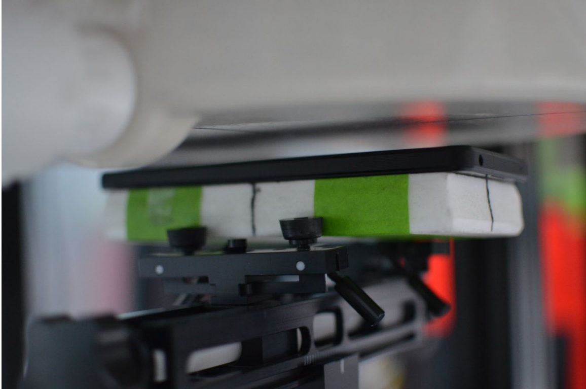
SAR Test Setup Photo 5 – Body-worn/Hotspot, Back Side at 10mm
