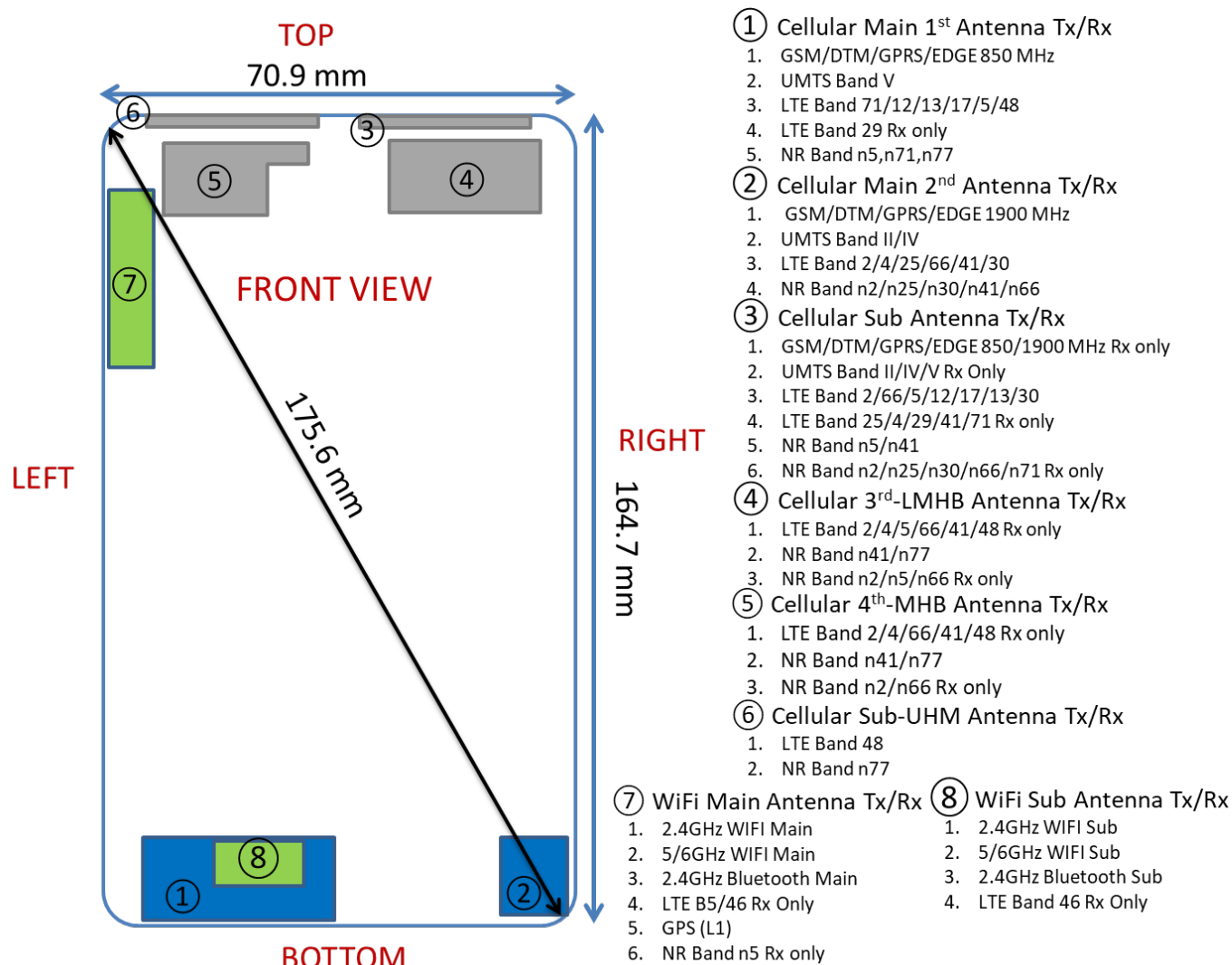
Figure J-1 DUT Antenna Locations
