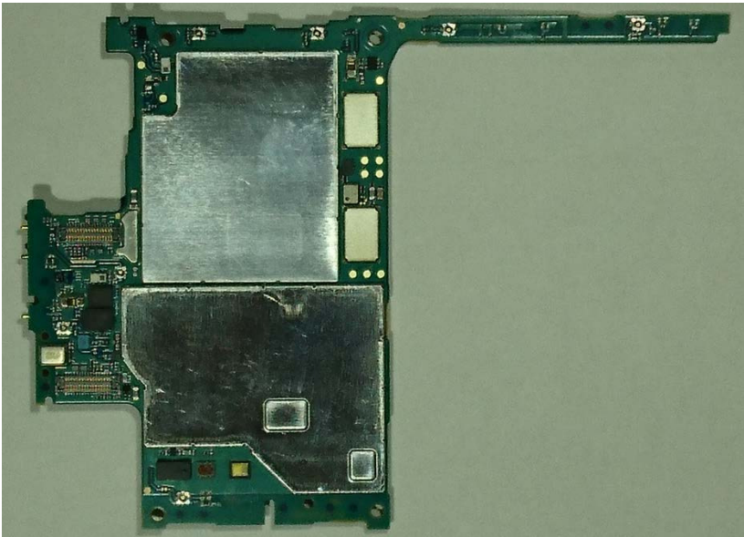
Internal PWB without Shield cases (Rear-side)
