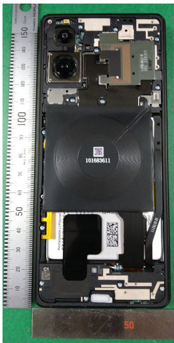
Without Rear panel
