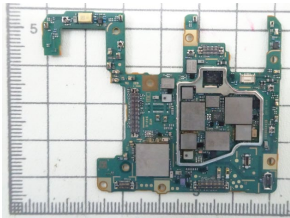
Rear PBA without Shield case (Front-side)
