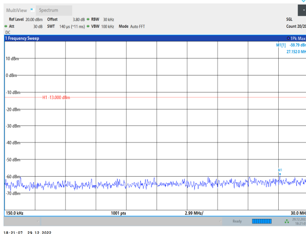
Band5-4132-0.15~30MHz
