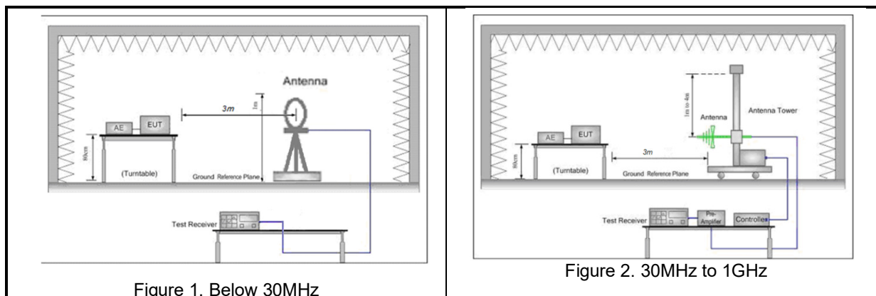
Figure 1. Below 30MHz
