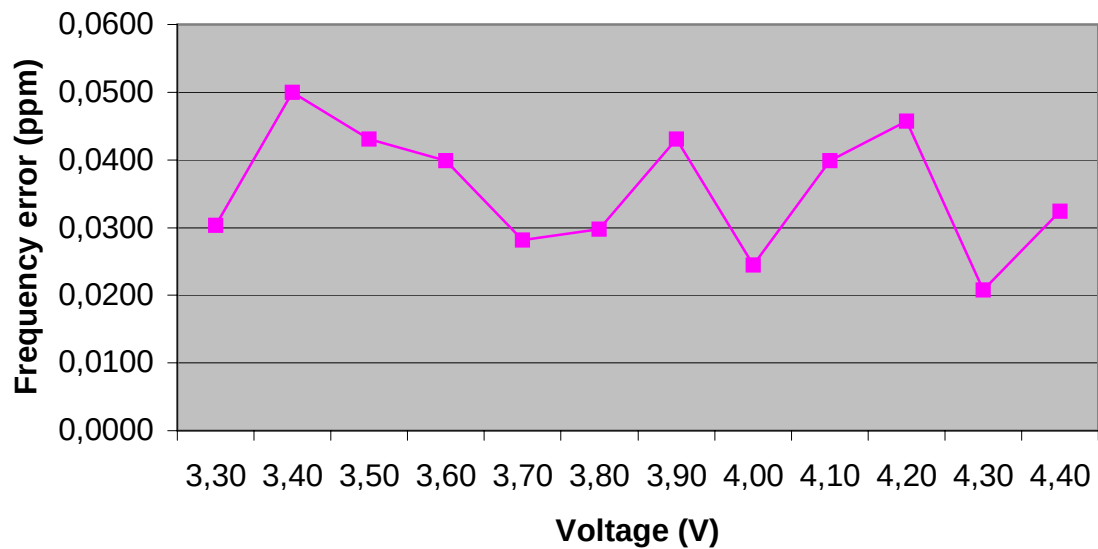
Frequency Error vs. Voltage
