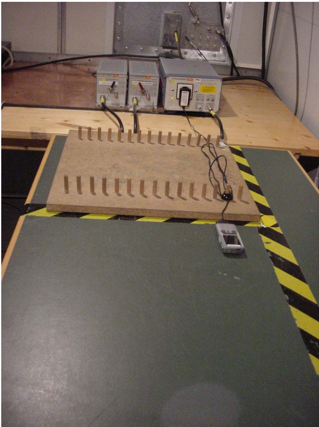
Photo 3 (Conducted Emissions):
