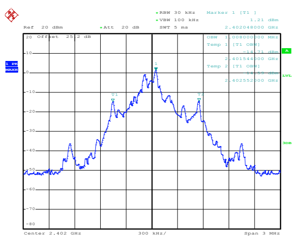
99% Bandwidth Plot on 2402MHz
