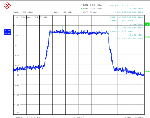
Highest Channel / 5MHz / 16QAM
