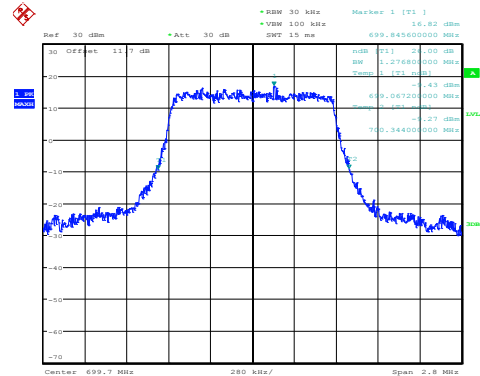
Lowest Channel / 1.4MHz / 16QAM
