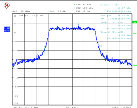
Highest Channel / 1.4MHz / 16QAM
