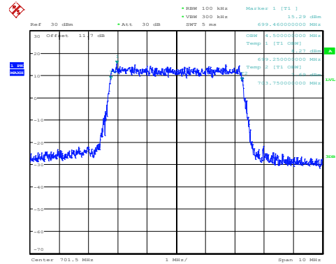
Lowest Channel / 5MHz / 16QAM
