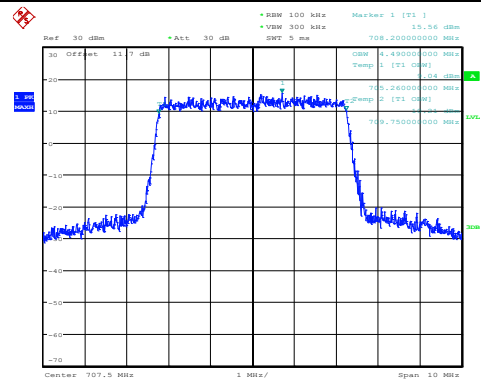
Middle Channel / 5MHz / 16QAM
