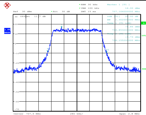
Middle Channel / 1.4MHz / 16QAM
