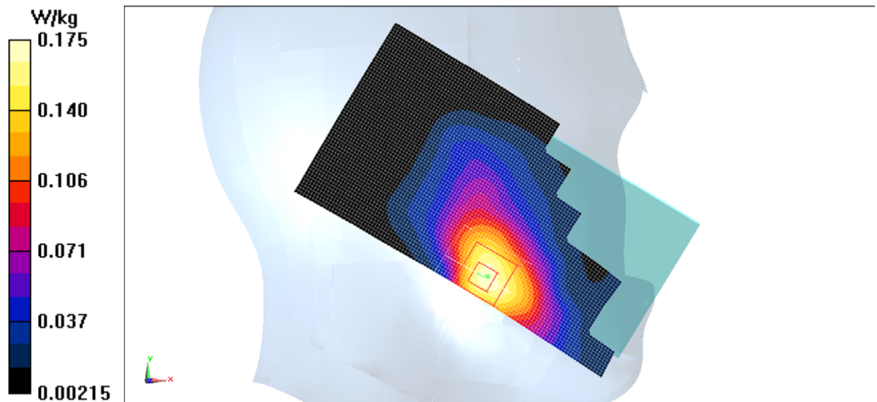
Fig.3 1900 MHz
