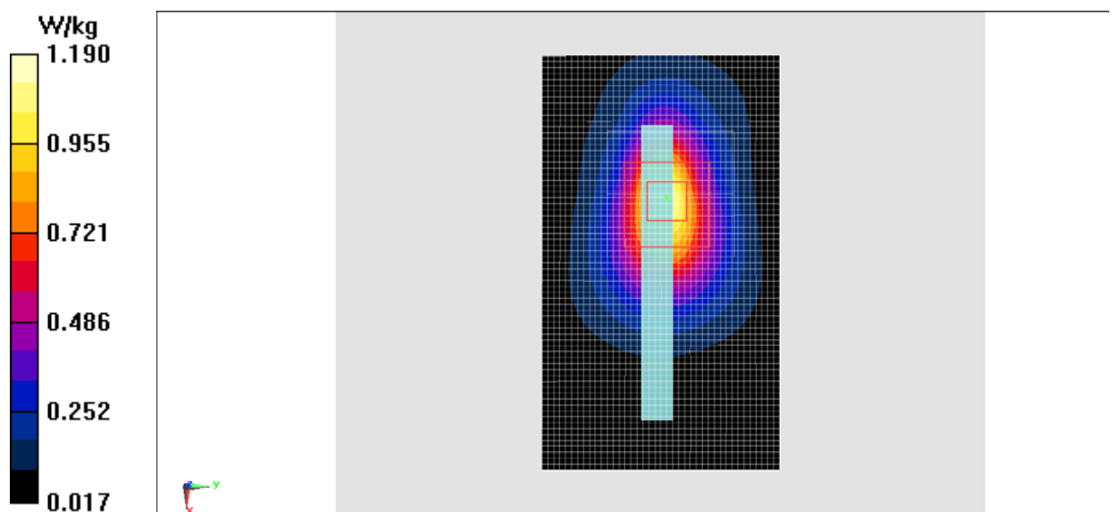
Fig.9 1700 MHz
