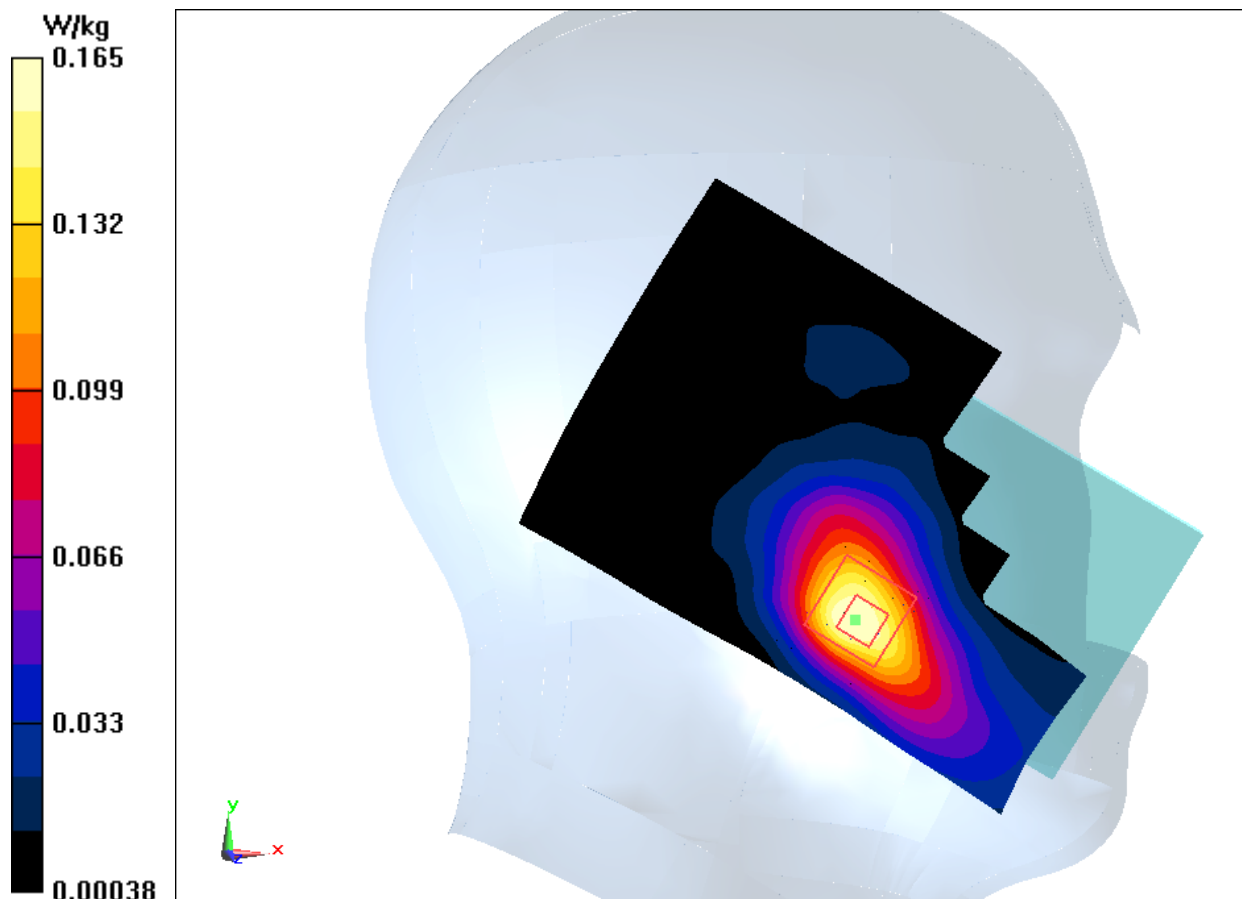
Fig.24 LTE Band41
