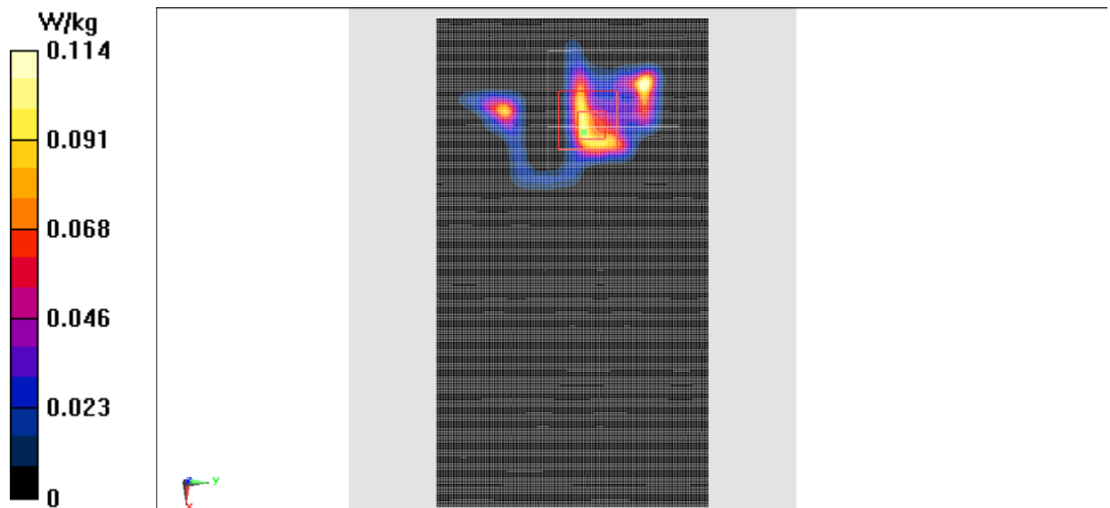
Fig.33 5GHz
