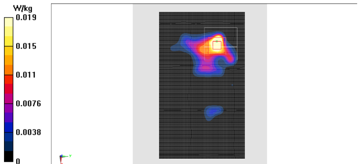
Fig.29 2450 MHz
