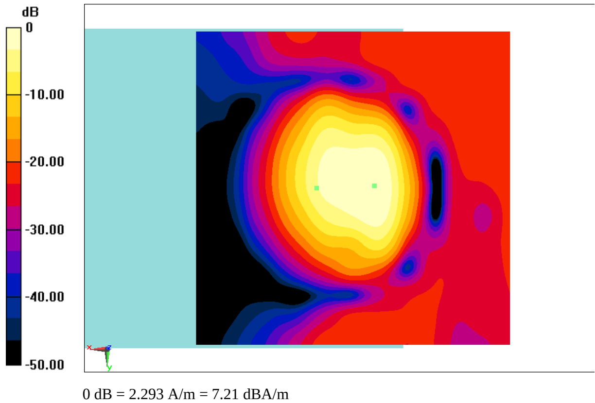
Fig B.10 T-Coil WCDMA 1900
