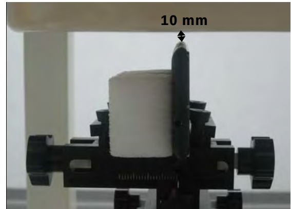
Fig.14 EUT right to flat phantom
