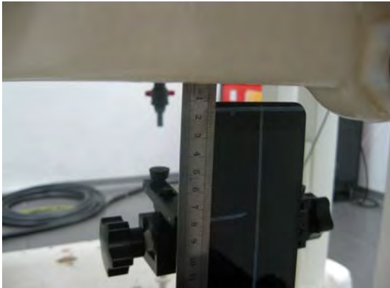
Fig.12 EUT top to flat phantom
