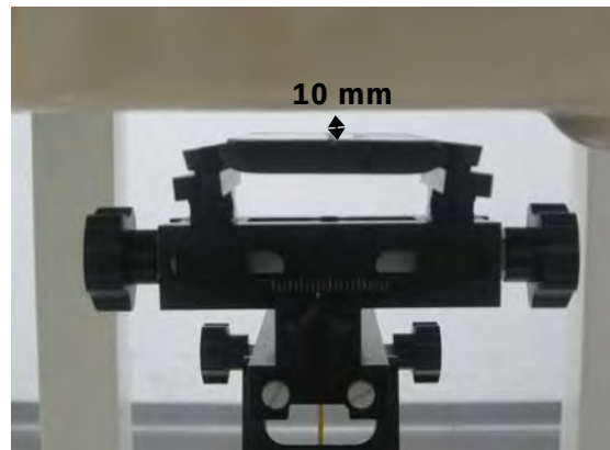
Fig.9 EUT front to flat phantom
