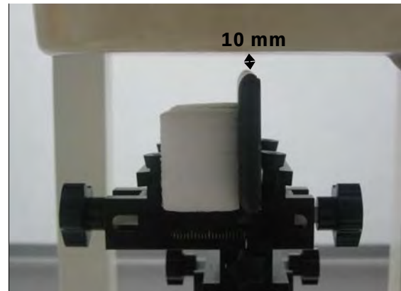
Fig.15 EUT left to flat phantom
