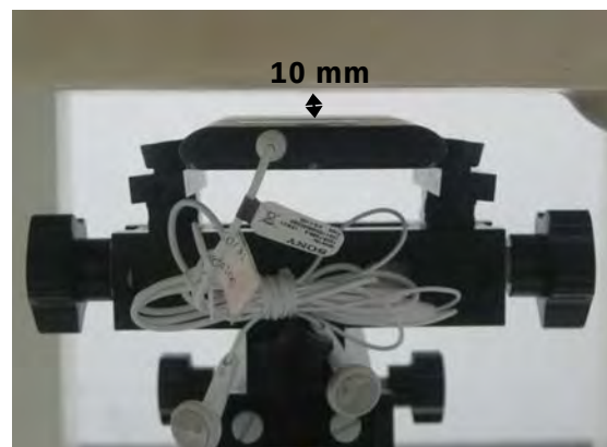
Fig.11 back side with headset to flat phantom
