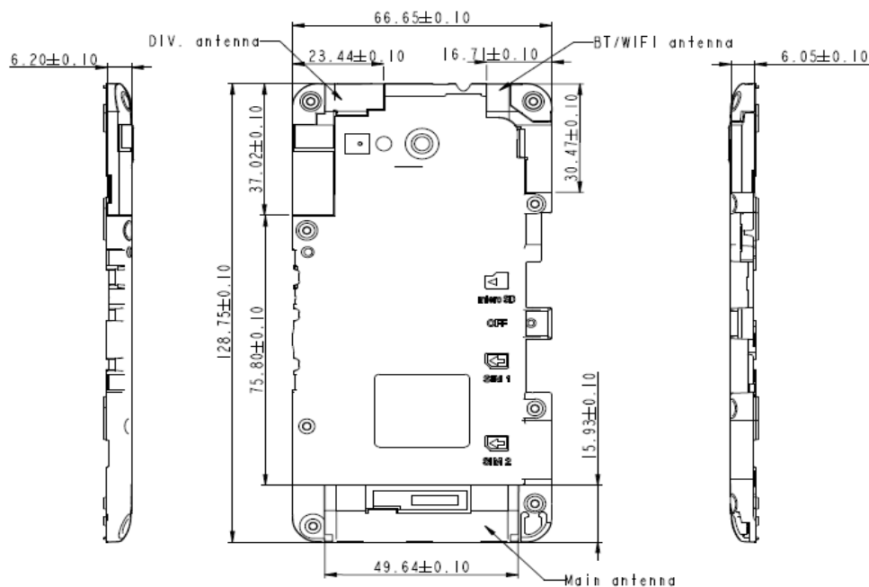
Fig.19 Antenna position of EUT
