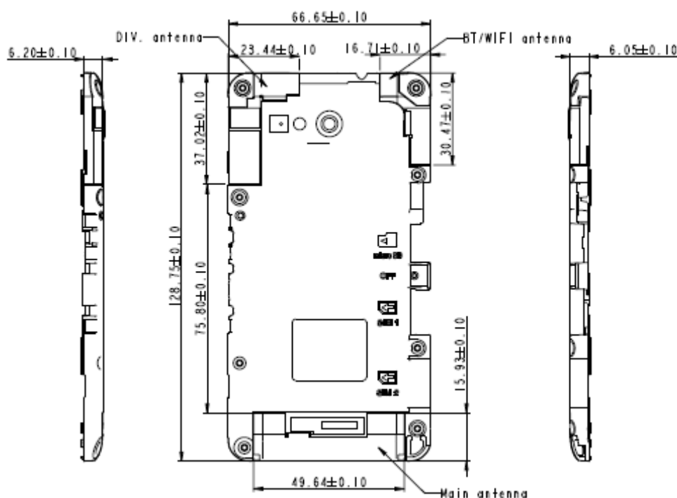
Fig.19 Antenna position of EUT - End of Report -
