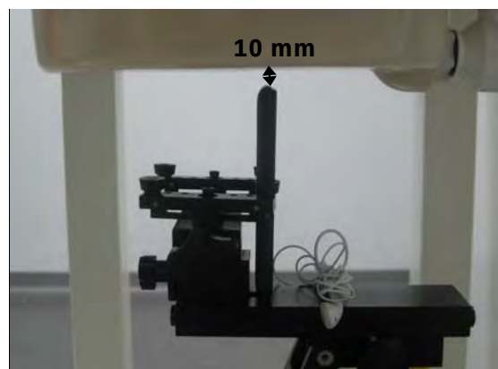
Fig.13 EUT bottom with headset to flat phantom
