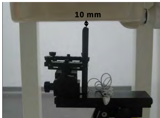
Fig.13 EUT bottom with headset to flat phantom
