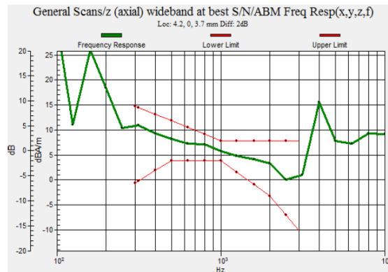
Fig 7.2 GSM1900 Ch661
