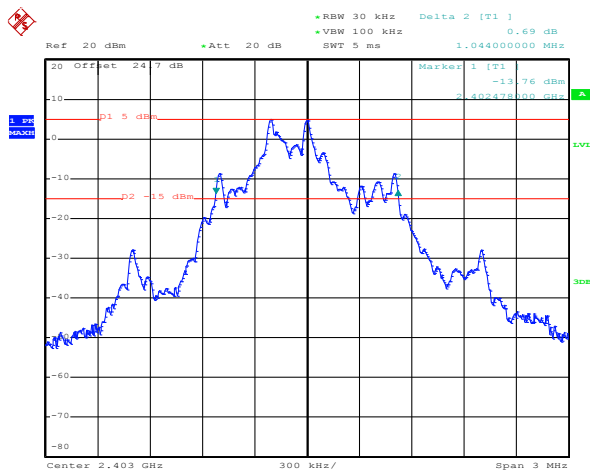
20 dB Bandwidth Plot on 2403MHz
