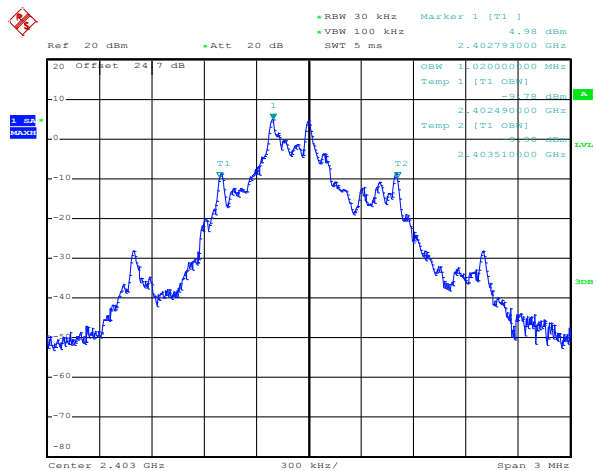
99% Bandwidth Plot on 2403MHz
