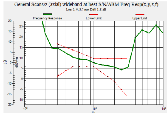
Fig 7.2 GSM1900 Ch661
