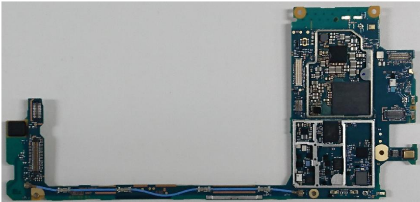
Internal PWB without Shield cases (Rear-side)
