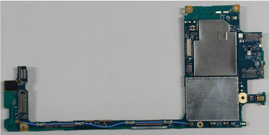
Internal PWB with Shield cases (Rear-side)
