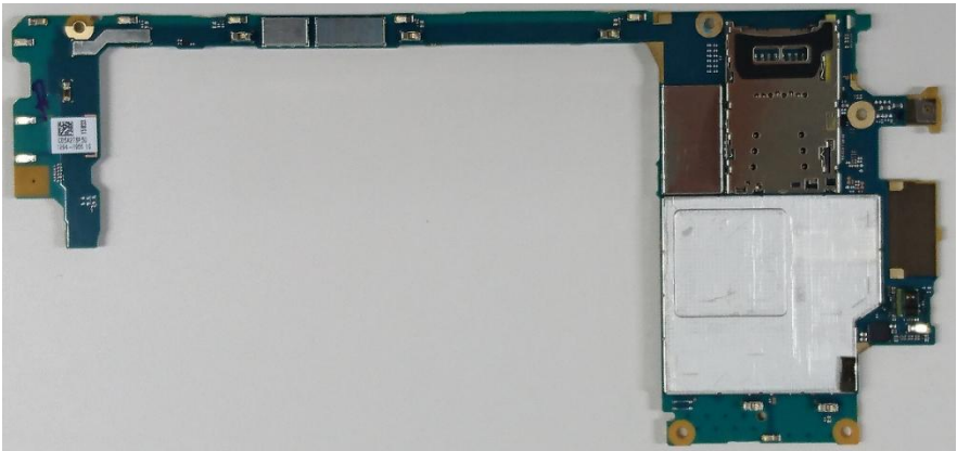
Internal PWB with Shield cases (Front-side)
