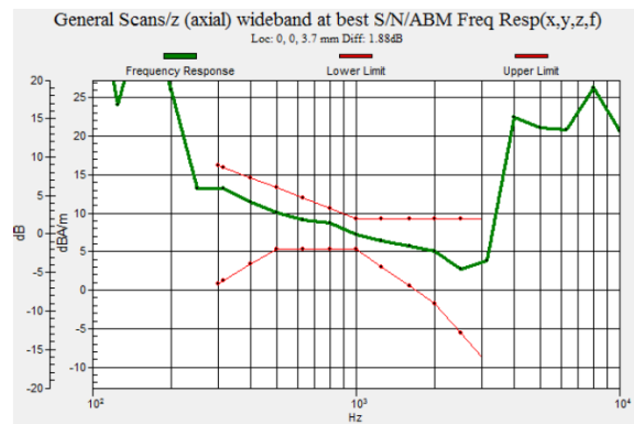
Fig 7.2 GSM1900 Ch661
