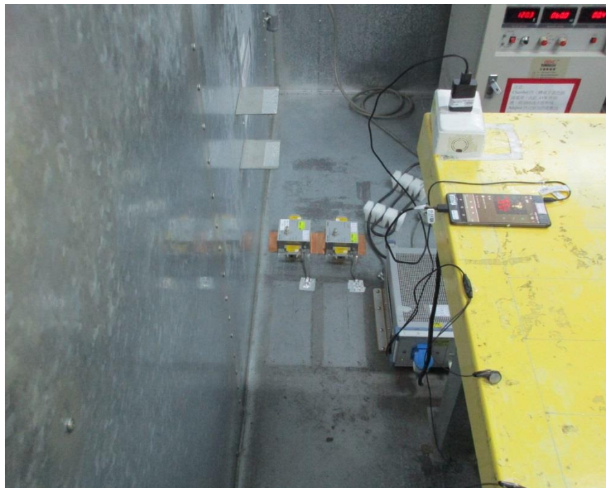
Rear View
