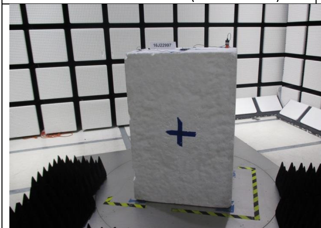
RADIATED FRONT PHOTO (ABOVE 1 GHz)
