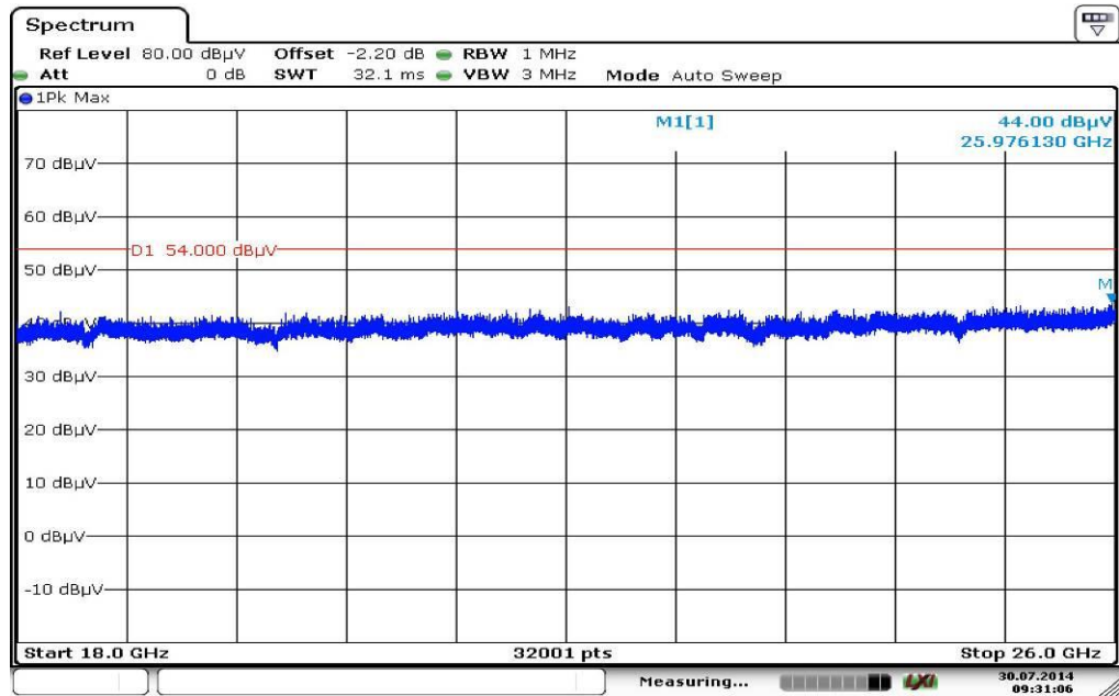
Plot 5: Receiver mode 18 GHz to 26 GHz
