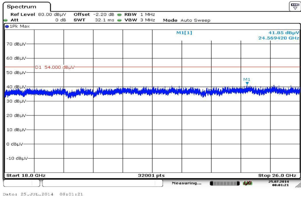
Plot 8: 18 GHz to 26 GHz, mid channel, vertical & horizontal polarization – valid for all channels
