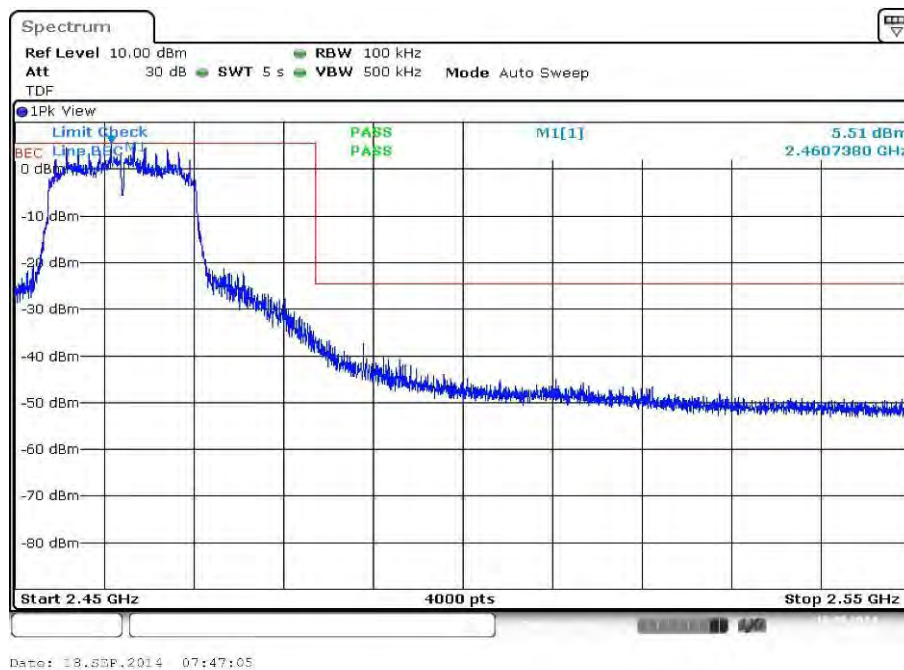
Plot 2: TX mode, upper band edge
