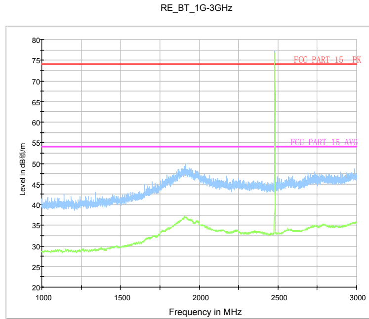
Fig.28. Radiated emission: GFSK, Channel 78, 1 GHz - 3 GHz
