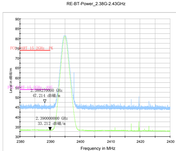
Fig.30. Radiated emission (Power): GFSK, low channel
