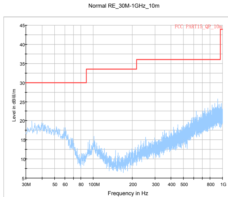
Fig.27. Radiated emission: GFSK, Channel 78, 30 MHz - 1 GHz
