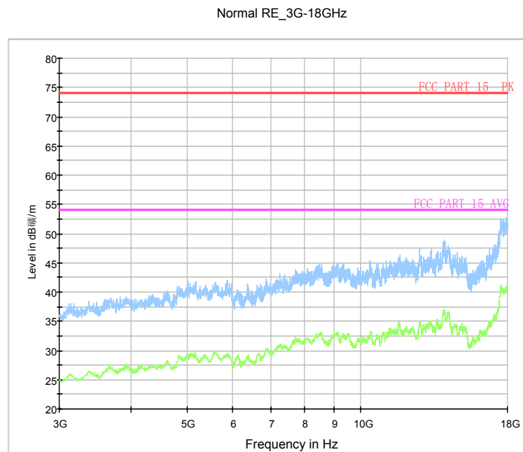
Fig.26. Radiated emission: GFSK, Channel 39, 3 GHz - 18 GHz
