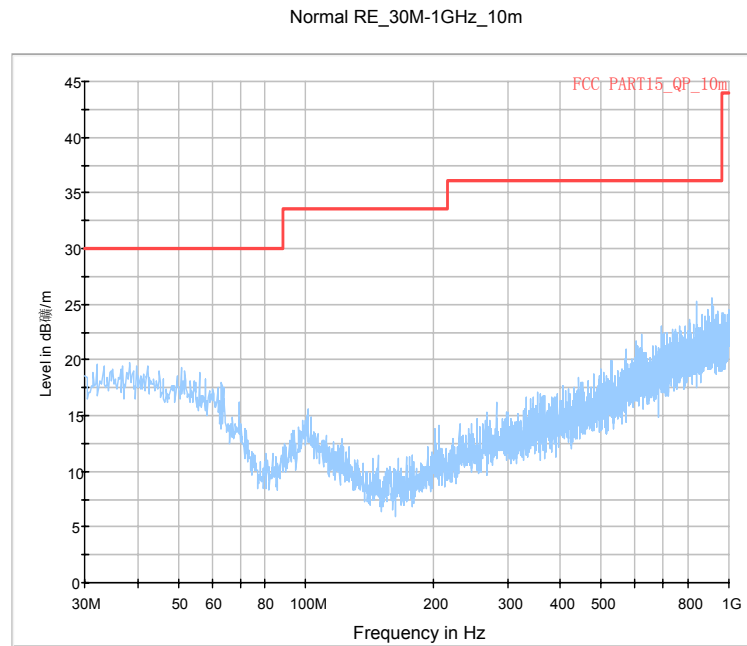
Fig.20. Radiated emission: GFSK, Channel 0, 30 MHz - 1 GHz
