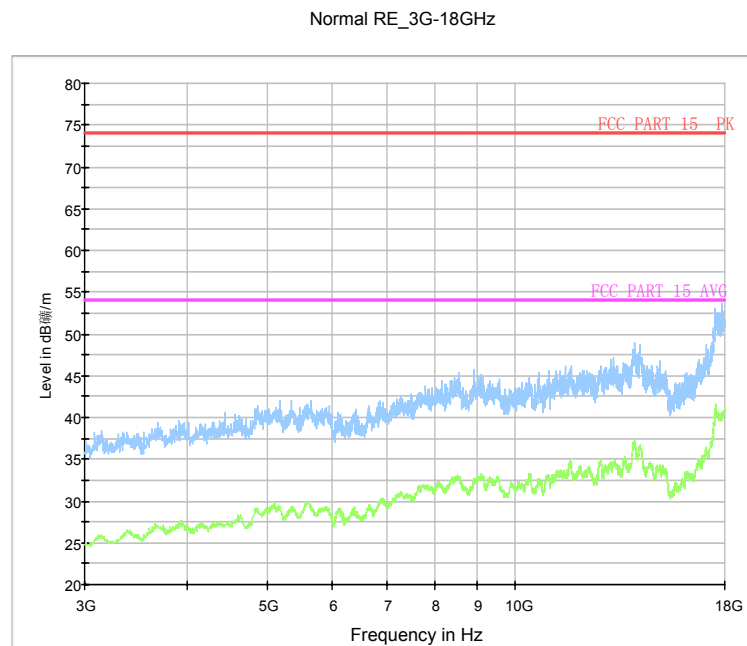
Fig.22. Radiated emission: GFSK, Channel 0, 3 GHz - 18 GHz
