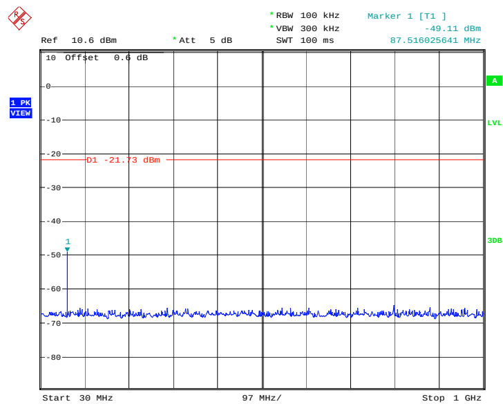
Fig.5. Conducted spurious emission: GFSK, Channel 0, 2402 MHz
