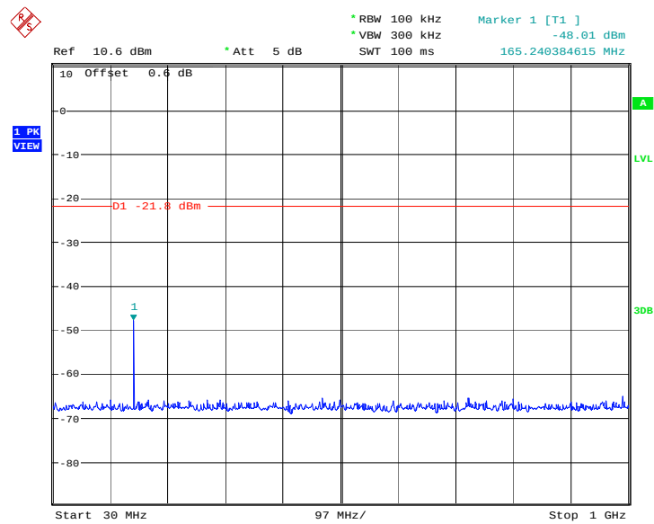
Fig.15. Conducted spurious emission: GFSK, Channel 78, 2480MHz
