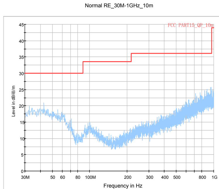
Fig.24. Radiated emission: GFSK, Channel 39, 30 MHz - 1 GHz
