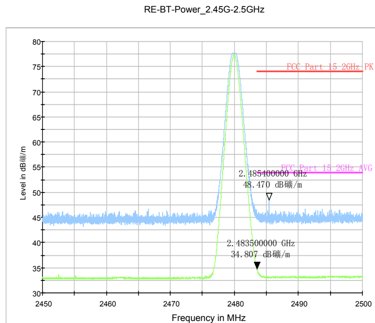
Fig.31. Radiated emission (Power) GFSK, high channel
