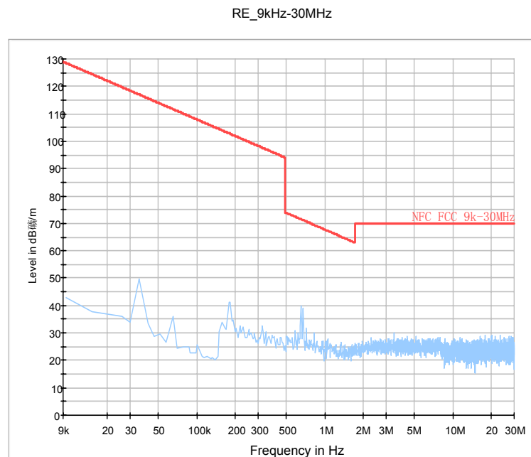
Fig.23. Radiated emission: GFSK, Channel 39, 9 kHz - 30 MHz
