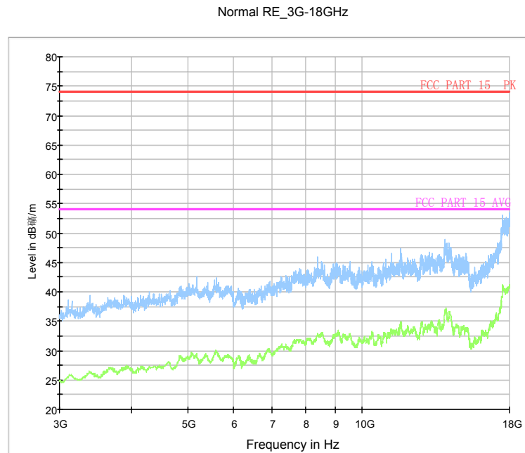
Fig.29. Radiated emission: GFSK, Channel 78, 3 GHz - 18 GHz
