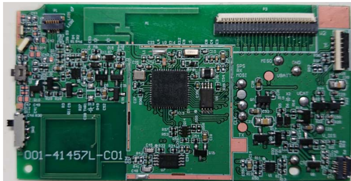
<RF board top side photo without shield>
