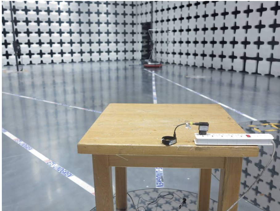
Picture C-1: Radiated emission
