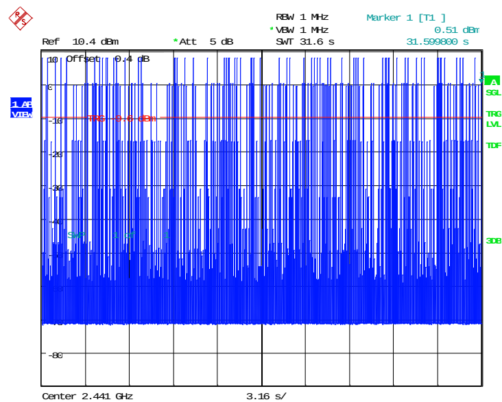
Fig.64. Time of occupancy (Dwell Time): Channel 39, GFSK-DH5
