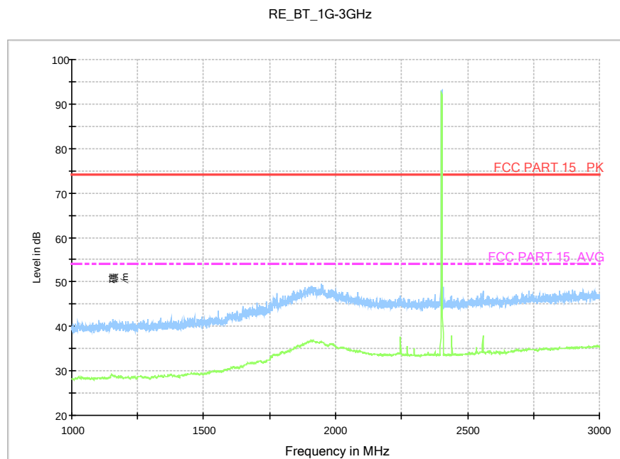
Fig.39. Radiated emission: GFSK, Channel 0, 1 GHz - 3 GHz
