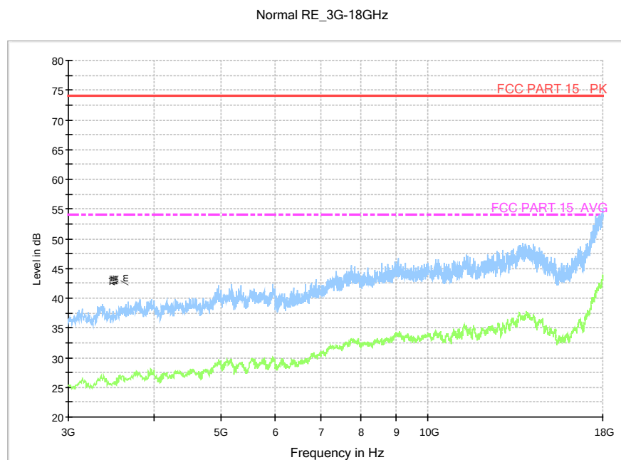
Fig.44. Radiated emission: GFSK, Channel 39, 3 GHz - 18 GHz
