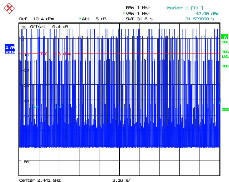
Fig.70. Time of occupancy (Dwell Time): Channel 39, \pi/4 DQPSK -DH5
