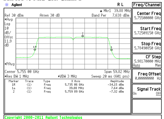
11n HT40 Mid CH. Chain 1
