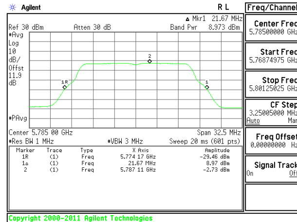
11n HT20 Mid CH. Chain 0
