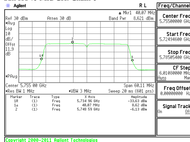
11n HT40 Mid CH. Chain 0
