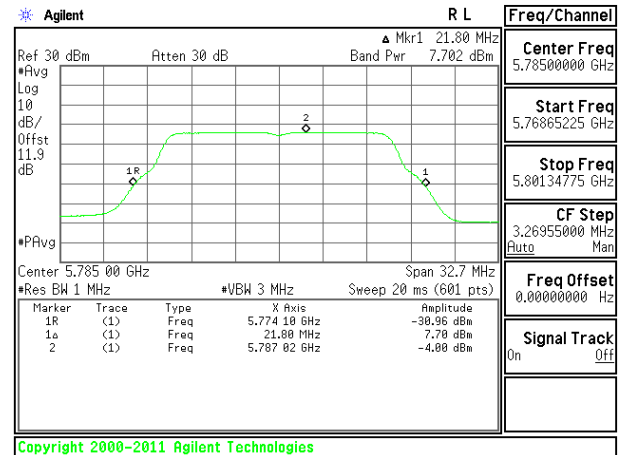
11n HT20 Mid CH. Chain 1
