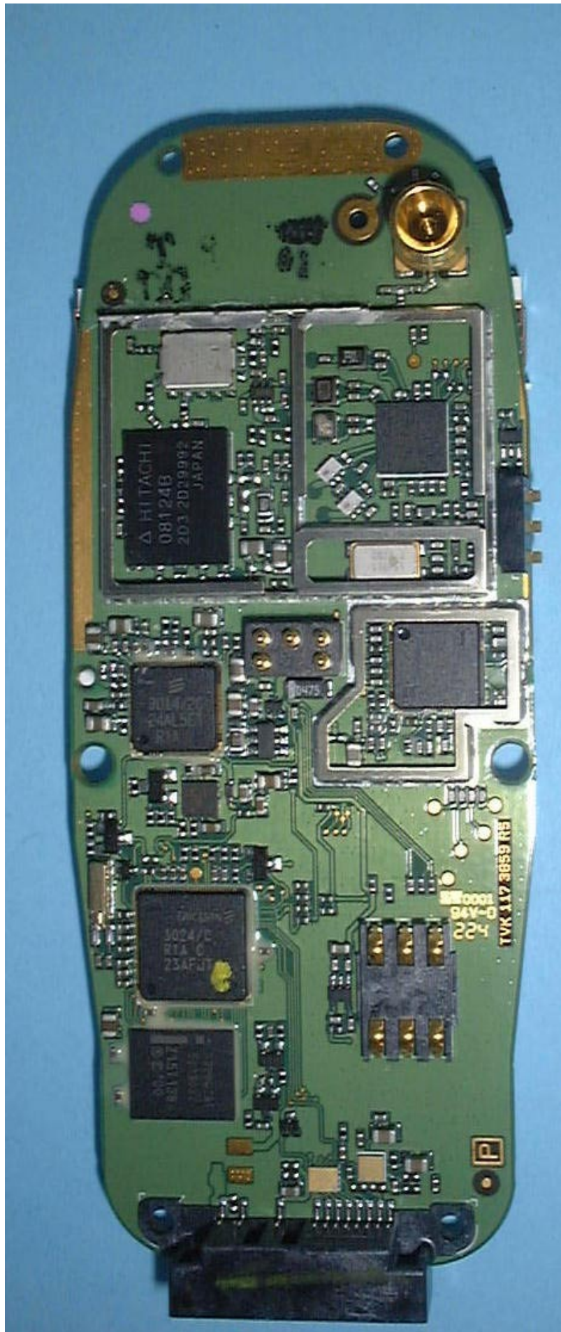
Rear view without shielding
