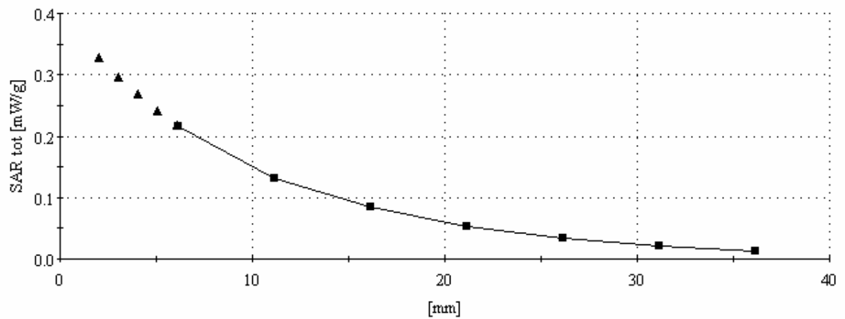
Z(x) distribution of max SAR in GSM1900 mode at 1850.2MHz. Measured against the head for cheek phone position
