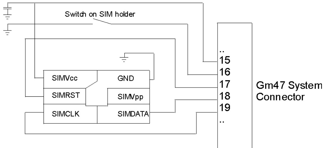
Figure 3.2 SIM Connections
