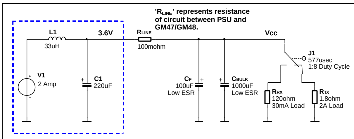
Figure 3.2 - Simplified Power Supply Reference Model
