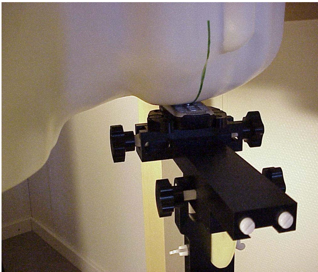
Device position against the head cheek phone position
