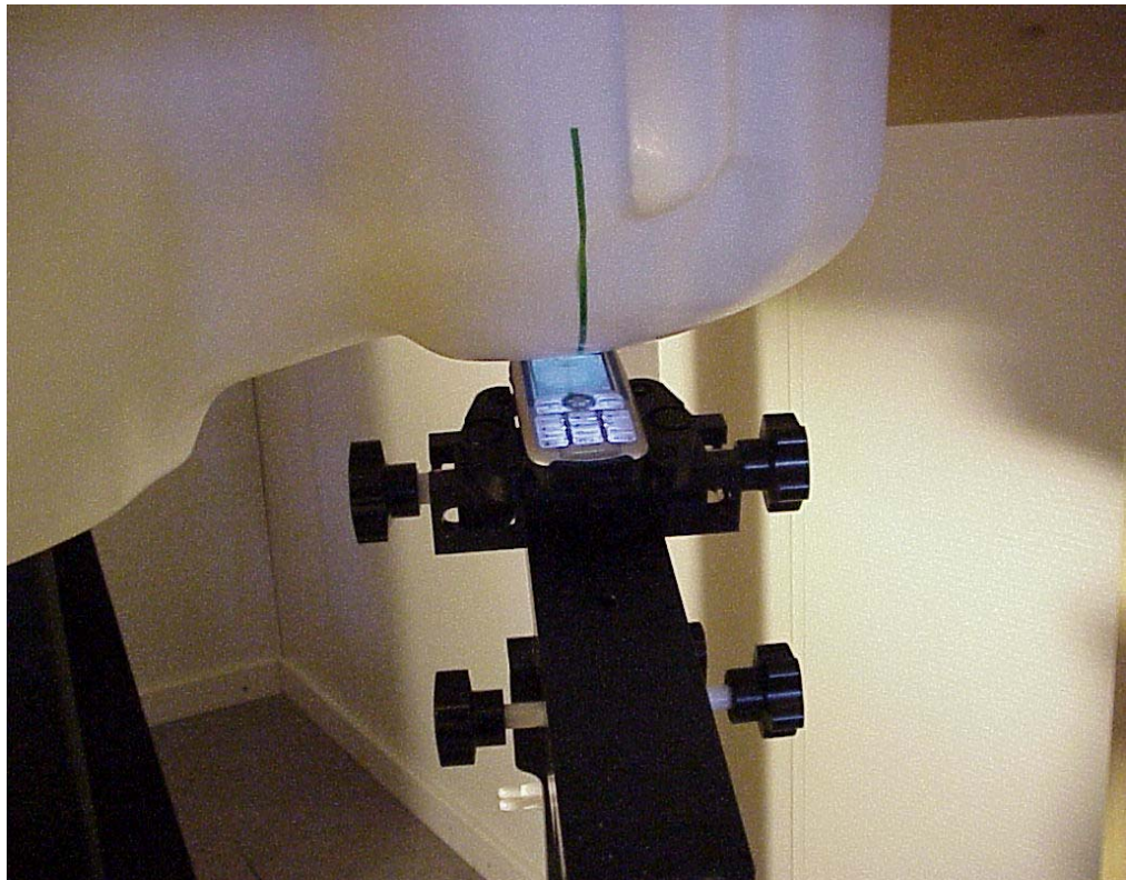
Device position against the head: Tilt phone position
