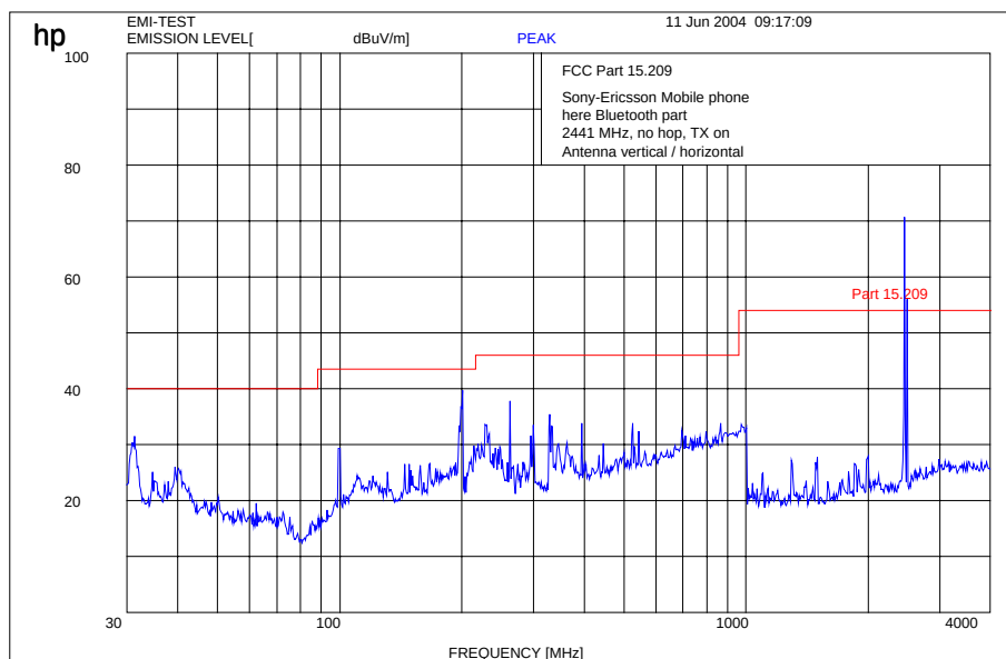
Plot 4 of 9: 0.03 - 4 GHz vertical/horizontal (middle channel)
