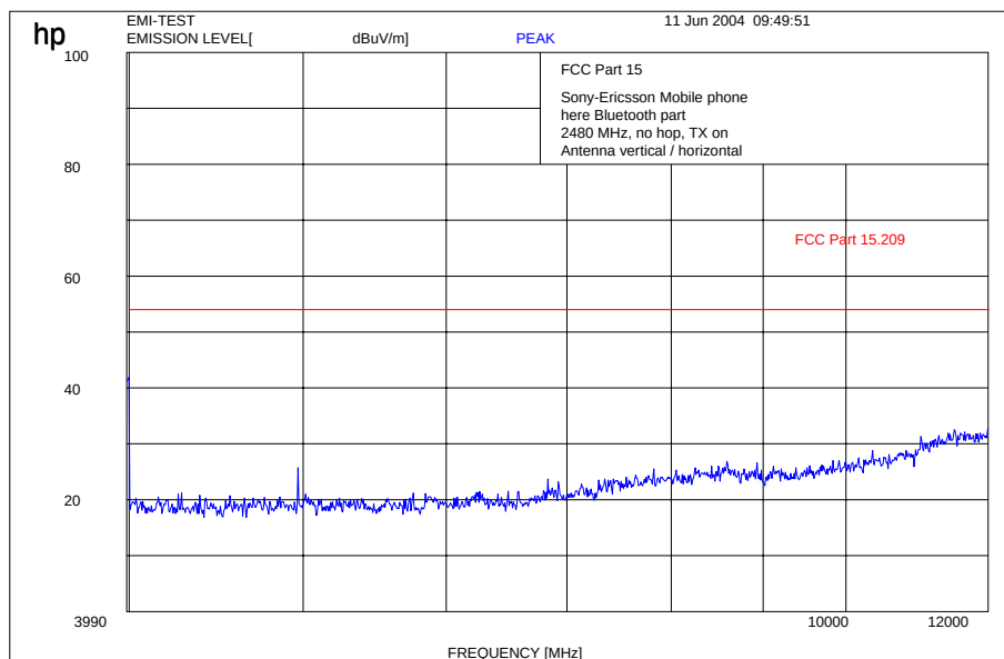
Plot 8 of 9: 4- 12 GHz vertical/horizontal (highest channel)
