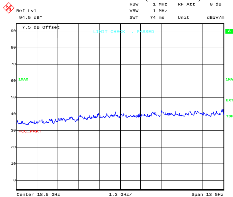
Plot 6 of 9: 12- 25 GHz vertical/horizontal (middle channel)
