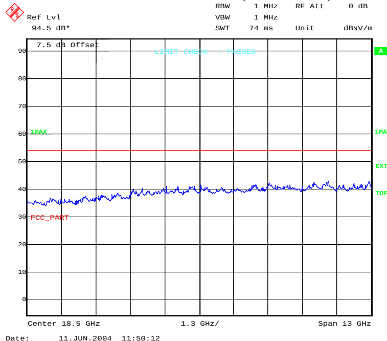
Plot 3 of 9: 12- 25 GHz vertical/horizontal (lowest channel)
