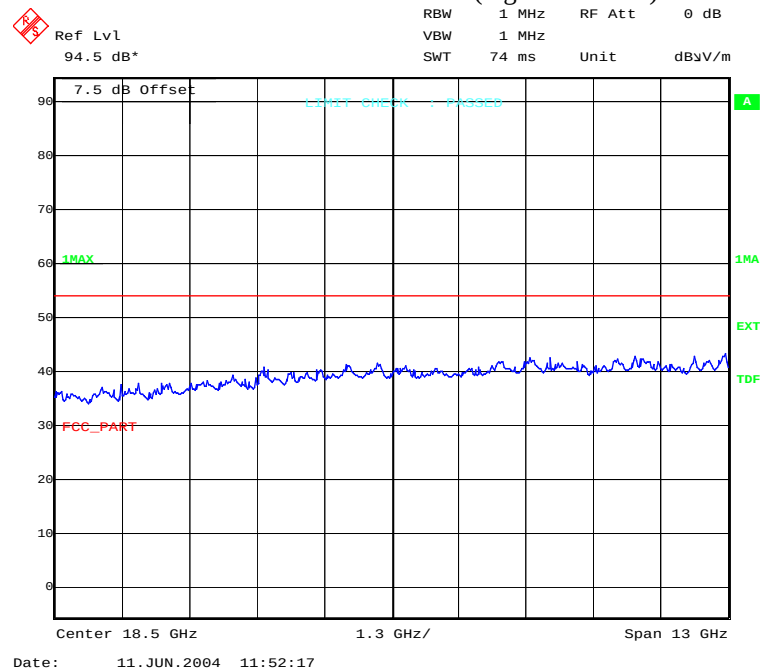
Plot 9 of 9: 12- 25 GHz vertical/horizontal (highest channel)
