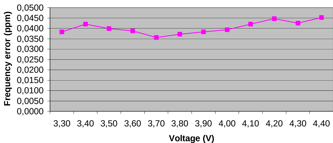
Frequency Error vs. Voltage
