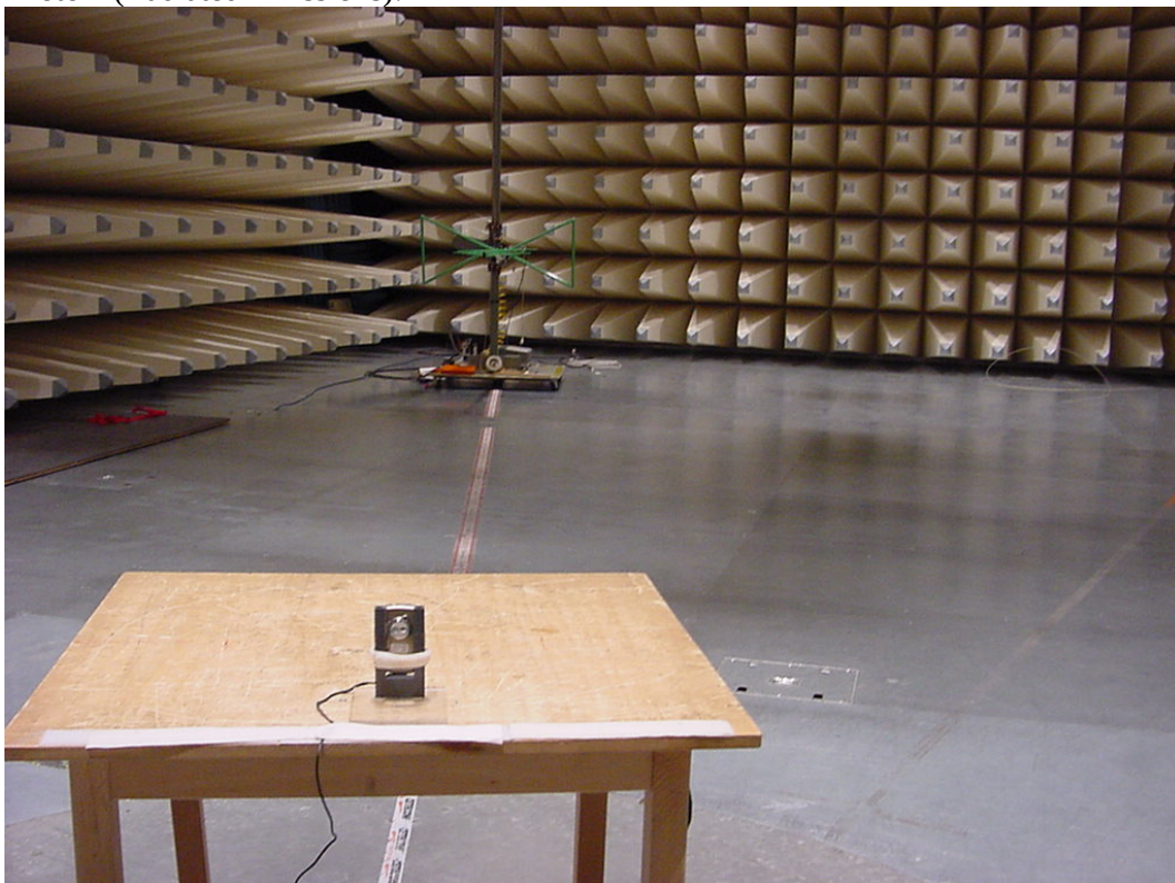
Photo 4 (Radiated Emissions):
