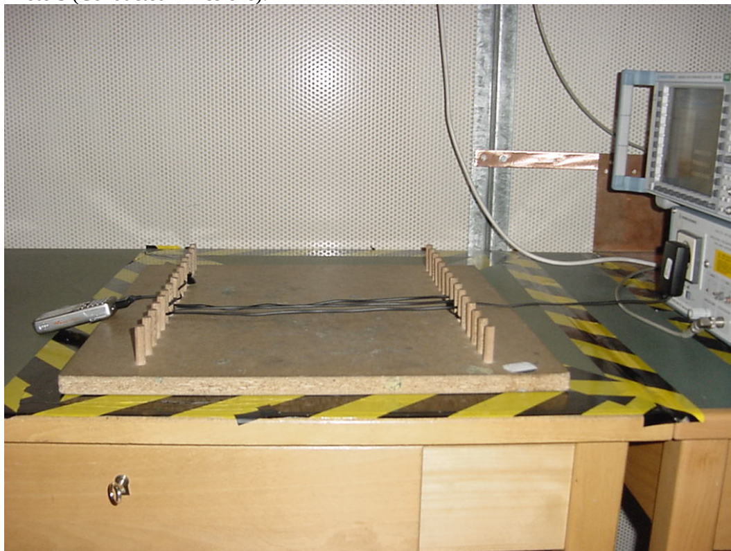
Photo 5 (Conducted Emissions):
