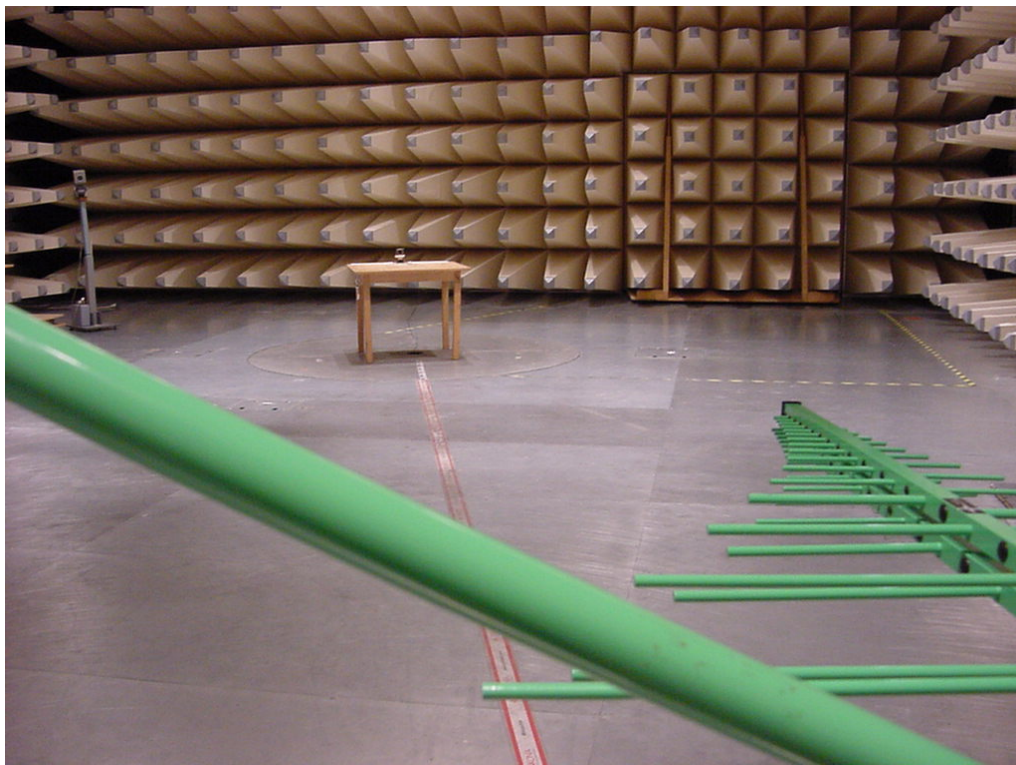
Photo 3: Radiated Emissions
