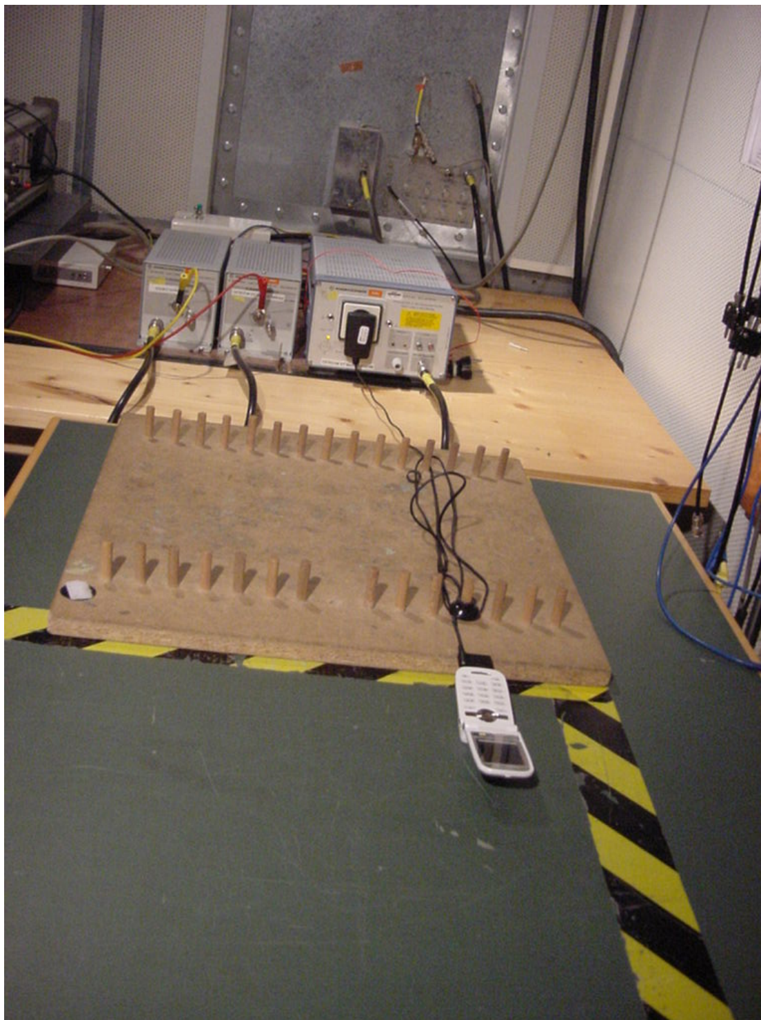
Photo 3 (Conducted Emissions):
