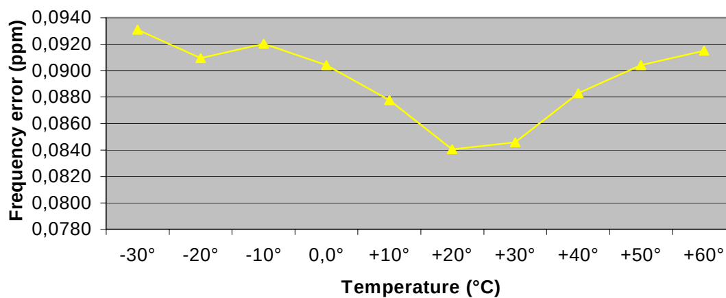
FREQUENCY ERROR VERSUS TEMPERATURE
